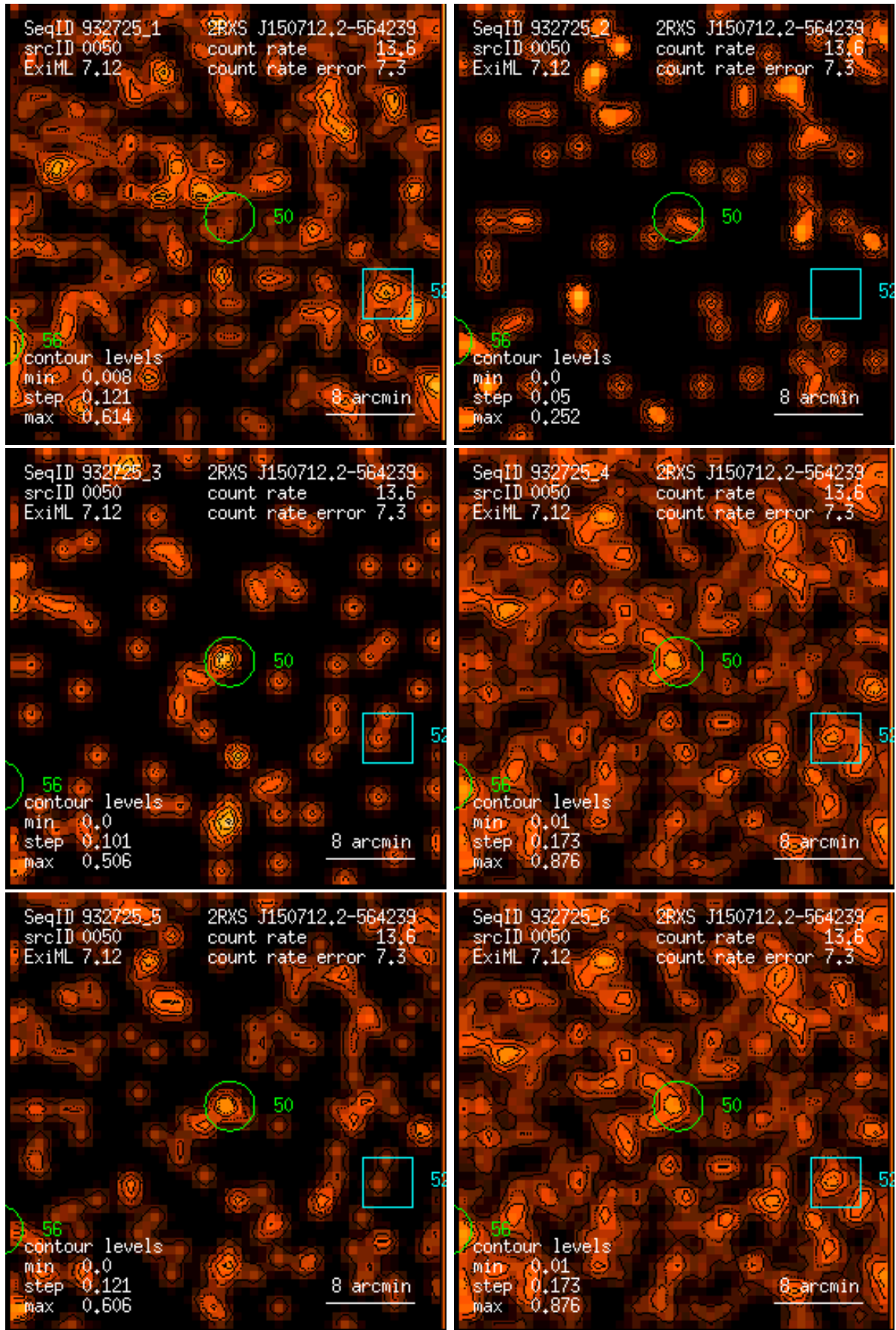
Figure 50: RASS 932725: detection 0050: band rate images, Gaussian filter: (1) PSPC channels 11 – 41, (2) 52 – 90, (3) 91 – 201, (4) 11 – 235, (5) 52 – 201, (6) 11 – 201. Broad band rates in counts/ks. Band rate contour levels in counts/ks/arcmin 2 .
