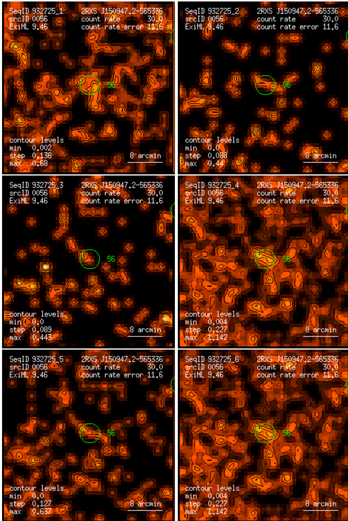
Figure 56: RASS 932725: detection 0056: band rate images, Gaussian filter: (1) PSPC channels 11 – 41, (2) 52 – 90, (3) 91 – 201, (4) 11 – 235, (5) 52 – 201, (6) 11 – 201. Broad band rates in counts/ks. Band rate contour levels in counts/ks/arcmin 2 .
