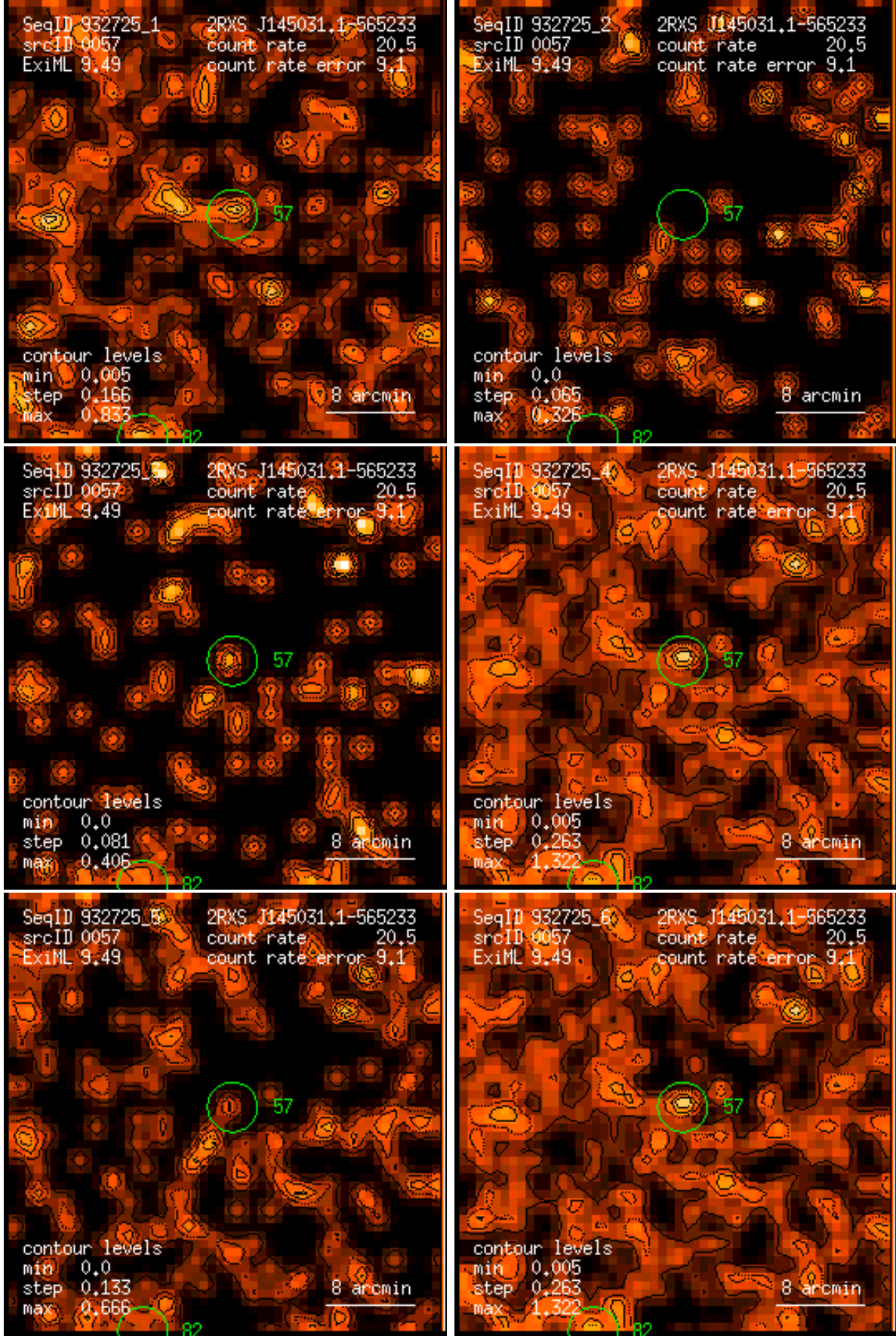
Figure 57: RASS 932725: detection 0057: band rate images, Gaussian filter: (1) PSPC channels 11 – 41, (2) 52 – 90, (3) 91 – 201, (4) 11 – 235, (5) 52 – 201, (6) 11 – 201. Broad band rates in counts/ks. Band rate contour levels in counts/ks/arcmin 2 .
