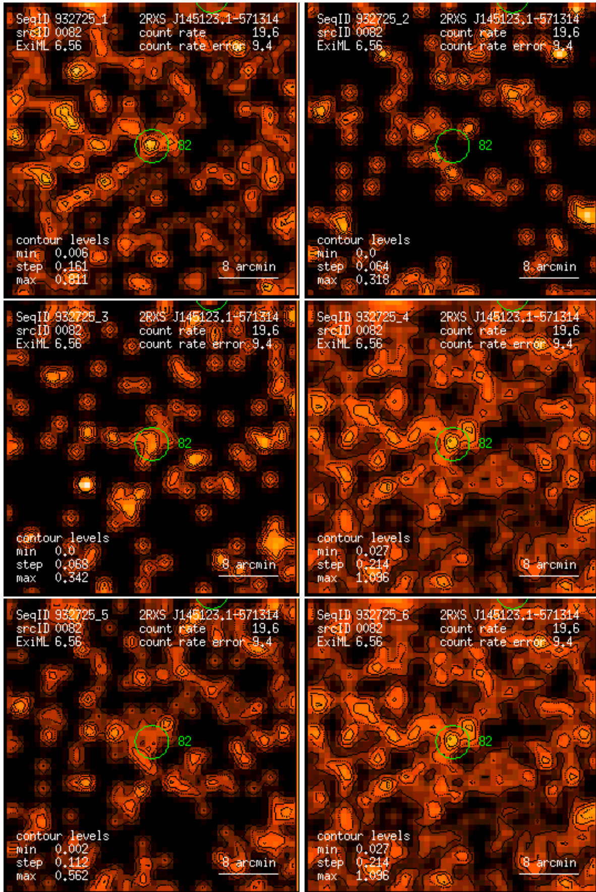
Figure 82: RASS 932725: detection 0082: band rate images, Gaussian filter: (1) PSPC channels 11 – 41, (2) 52 – 90, (3) 91 – 201, (4) 11 – 235, (5) 52 – 201, (6) 11 – 201. Broad band rates in counts/ks. Band rate contour levels in counts/ks/arcmin 2 .
