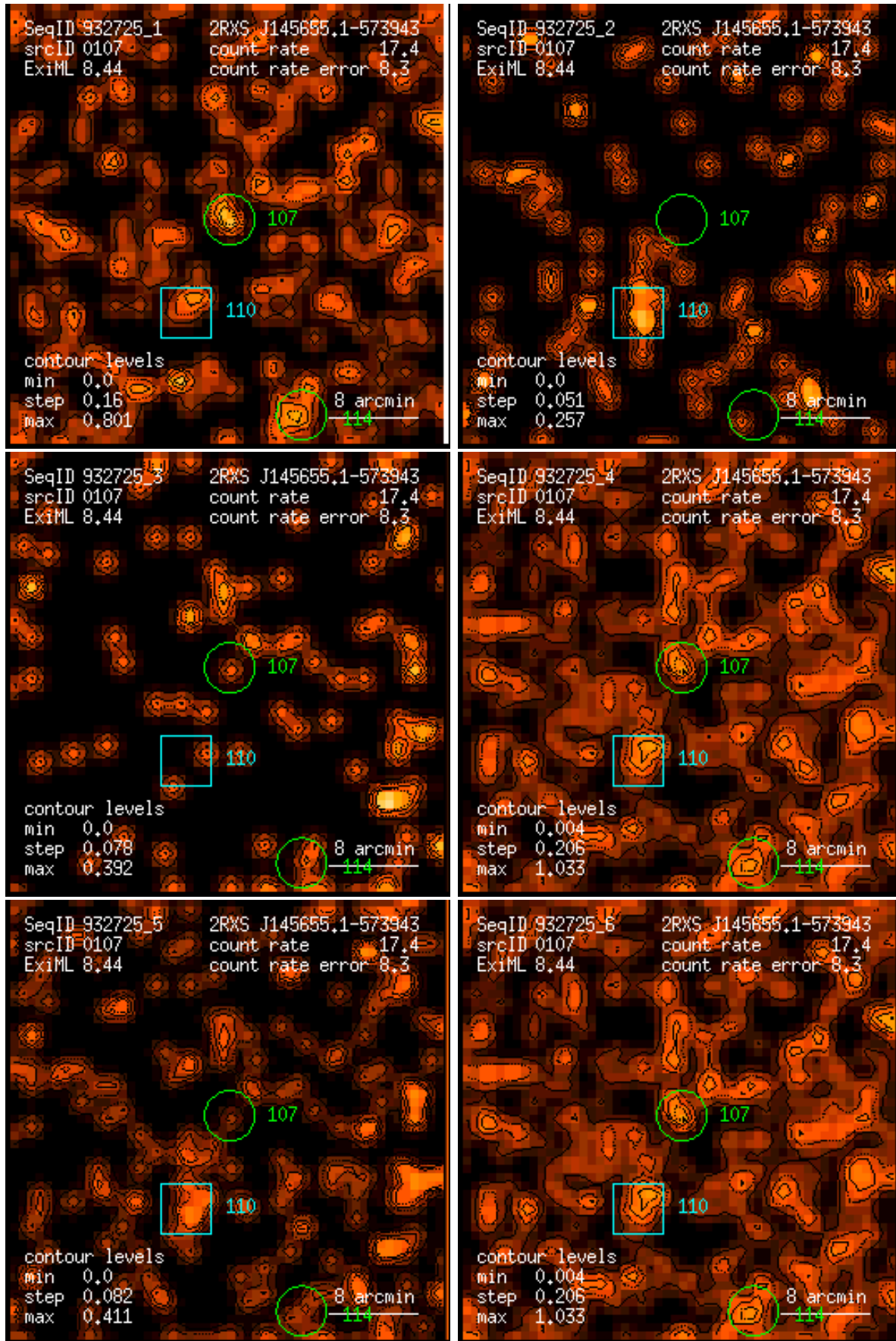
Figure 107: RASS 932725: detection 0107: band rate images, Gaussian filter: (1) PSPC channels 11 – 41, (2) 52 – 90, (3) 91 – 201, (4) 11 – 235, (5) 52 – 201, (6) 11 – 201. Broad band rates in counts/ks. Band rate contour levels in counts/ks/arcmin 2 .
