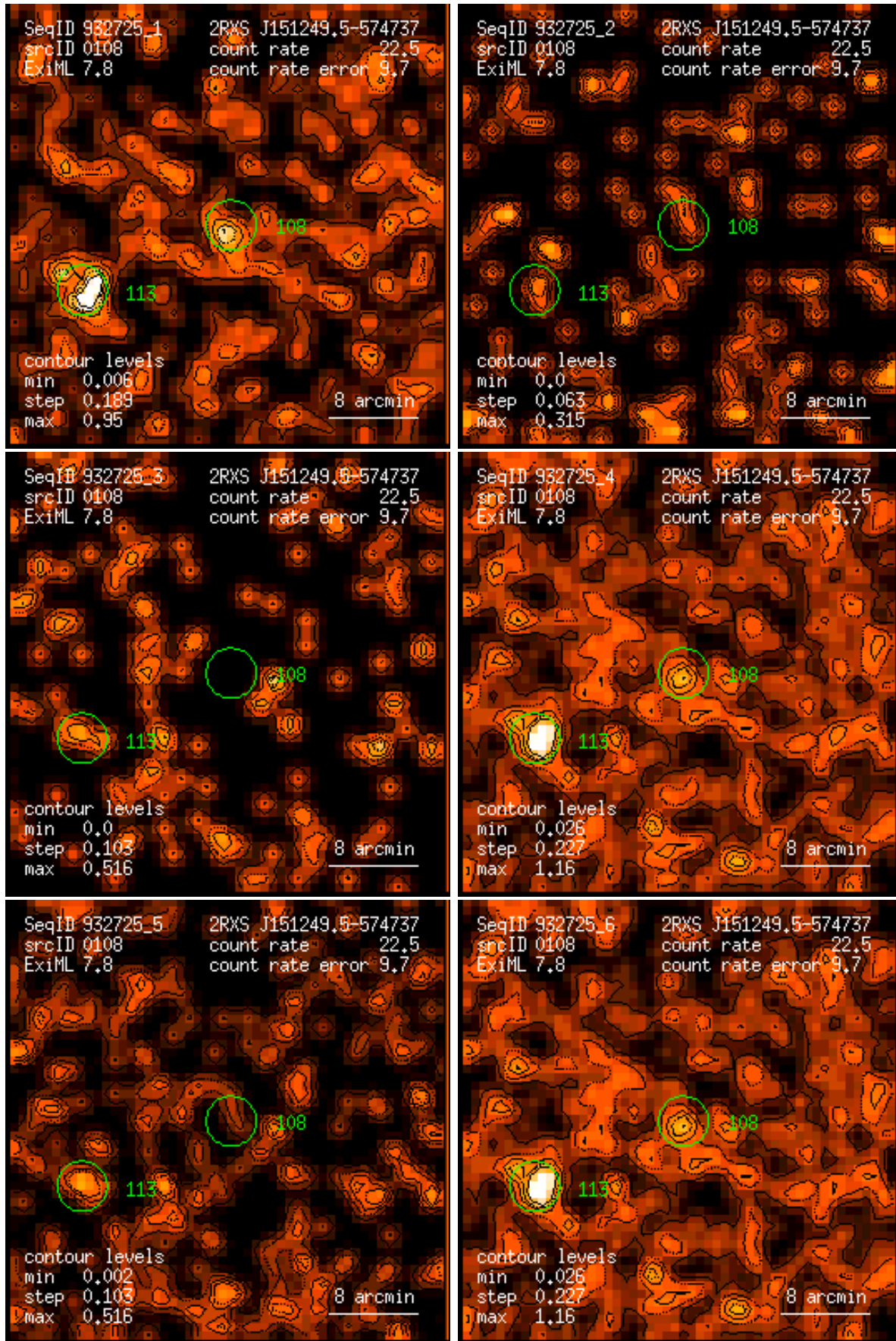
Figure 108: RASS 932725: detection 0108: band rate images, Gaussian filter: (1) PSPC channels 11 – 41, (2) 52 – 90, (3) 91 – 201, (4) 11 – 235, (5) 52 – 201, (6) 11 – 201. Broad band rates in counts/ks. Band rate contour levels in counts/ks/arcmin 2 .
