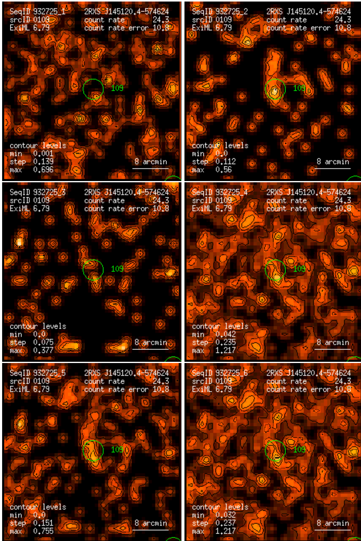
Figure 109: RASS 932725: detection 0109: band rate images, Gaussian filter: (1) PSPC channels 11 – 41, (2) 52 – 90, (3) 91 – 201, (4) 11 – 235, (5) 52 – 201, (6) 11 – 201. Broad band rates in counts/ks. Band rate contour levels in counts/ks/arcmin 2 .
