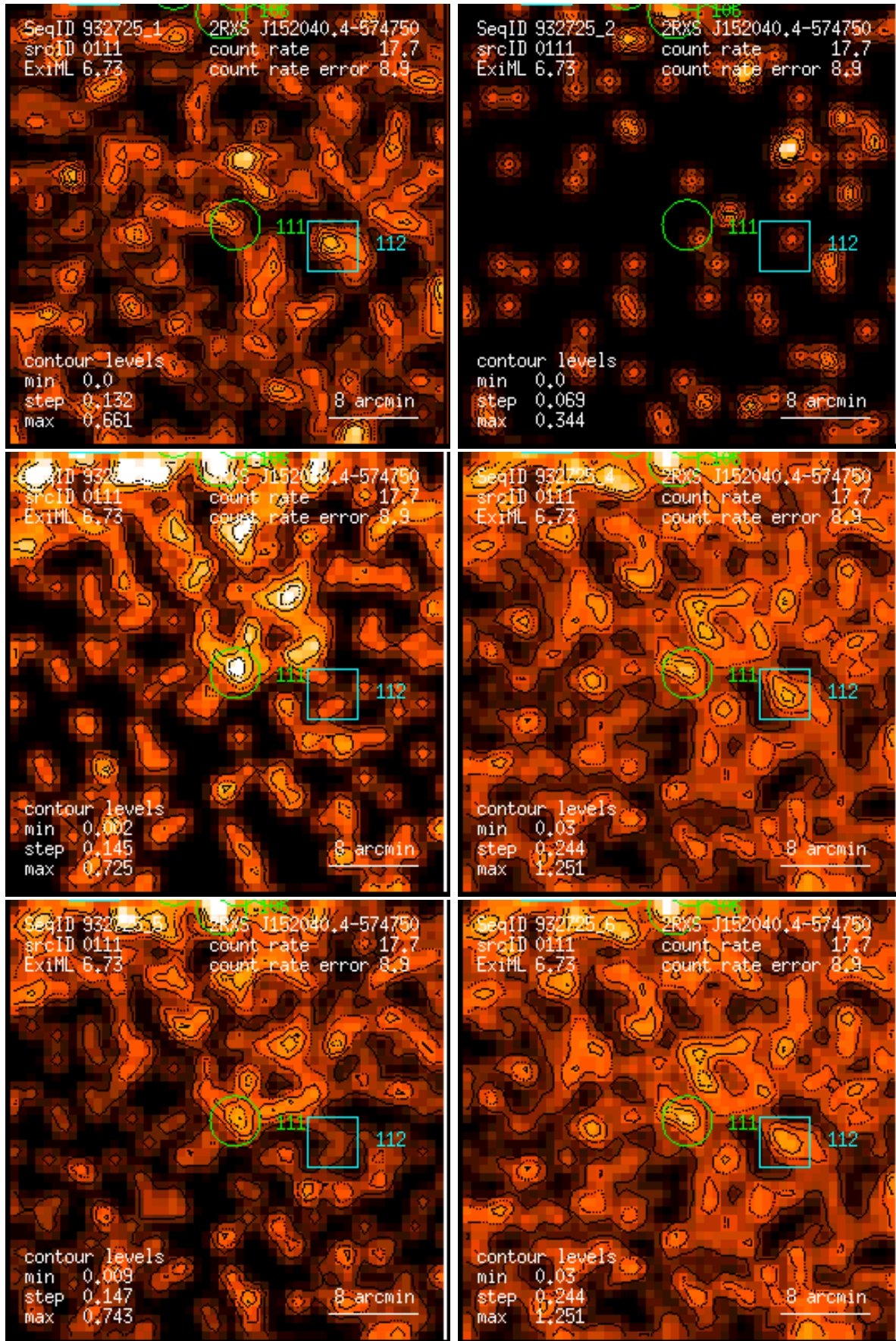
Figure 111: RASS 932725: detection 0111: band rate images, Gaussian filter: (1) PSPC channels 11 – 41, (2) 52 – 90, (3) 91 – 201, (4) 11 – 235, (5) 52 – 201, (6) 11 – 201. Broad band rates in counts/ks. Band rate contour levels in counts/ks/arcmin 2 .
