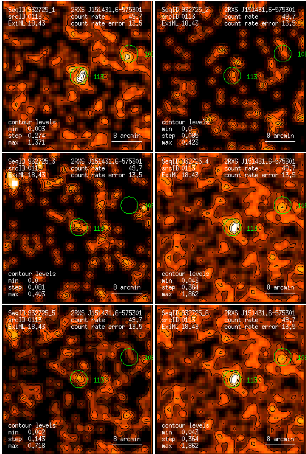
Figure 113: RASS 932725: detection 0113: band rate images, Gaussian filter: (1) PSPC channels 11 – 41, (2) 52 – 90, (3) 91 – 201, (4) 11 – 235, (5) 52 – 201, (6) 11 – 201. Broad band rates in counts/ks. Band rate contour levels in counts/ks/arcmin 2 .
