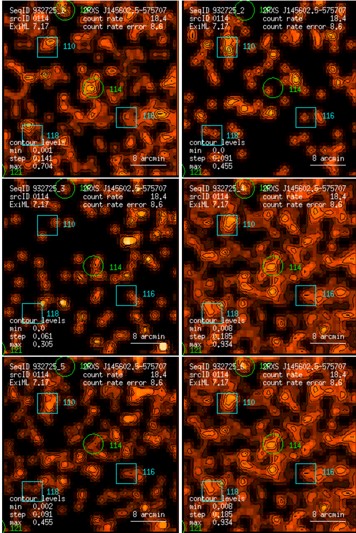
Figure 114: RASS 932725: detection 0114: band rate images, Gaussian filter: (1) PSPC channels 11 – 41, (2) 52 – 90, (3) 91 – 201, (4) 11 – 235, (5) 52 – 201, (6) 11 – 201. Broad band rates in counts/ks. Band rate contour levels in counts/ks/arcmin 2 .
