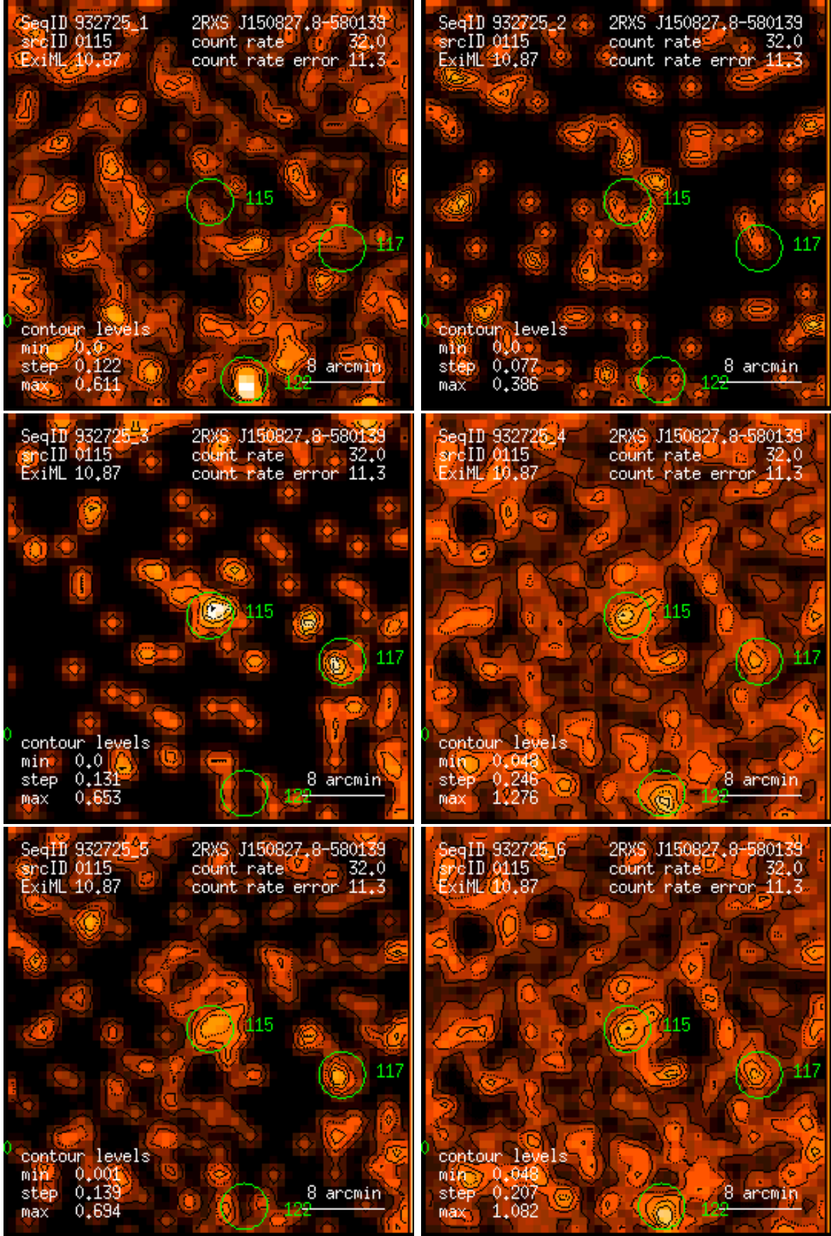
Figure 115: RASS 932725: detection 0115: band rate images, Gaussian filter: (1) PSPC channels 11 – 41, (2) 52 – 90, (3) 91 – 201, (4) 11 – 235, (5) 52 – 201, (6) 11 – 201. Broad band rates in counts/ks. Band rate contour levels in counts/ks/arcmin 2 .
