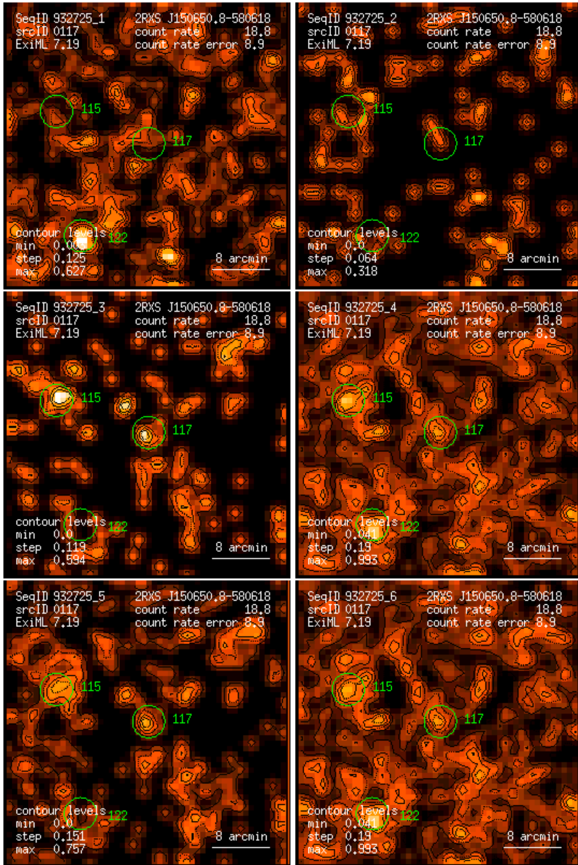
Figure 117: RASS 932725: detection 0117: band rate images, Gaussian filter: (1) PSPC channels 11 – 41, (2) 52 – 90, (3) 91 – 201, (4) 11 – 235, (5) 52 – 201, (6) 11 – 201. Broad band rates in counts/ks. Band rate contour levels in counts/ks/arcmin 2 .
