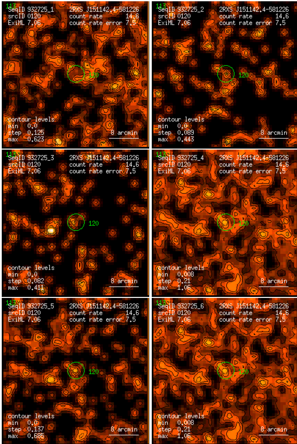
Figure 120: RASS 932725: detection 0120: band rate images, Gaussian filter: (1) PSPC channels 11 – 41, (2) 52 – 90, (3) 91 – 201, (4) 11 – 235, (5) 52 – 201, (6) 11 – 201. Broad band rates in counts/ks. Band rate contour levels in counts/ks/arcmin 2 .
