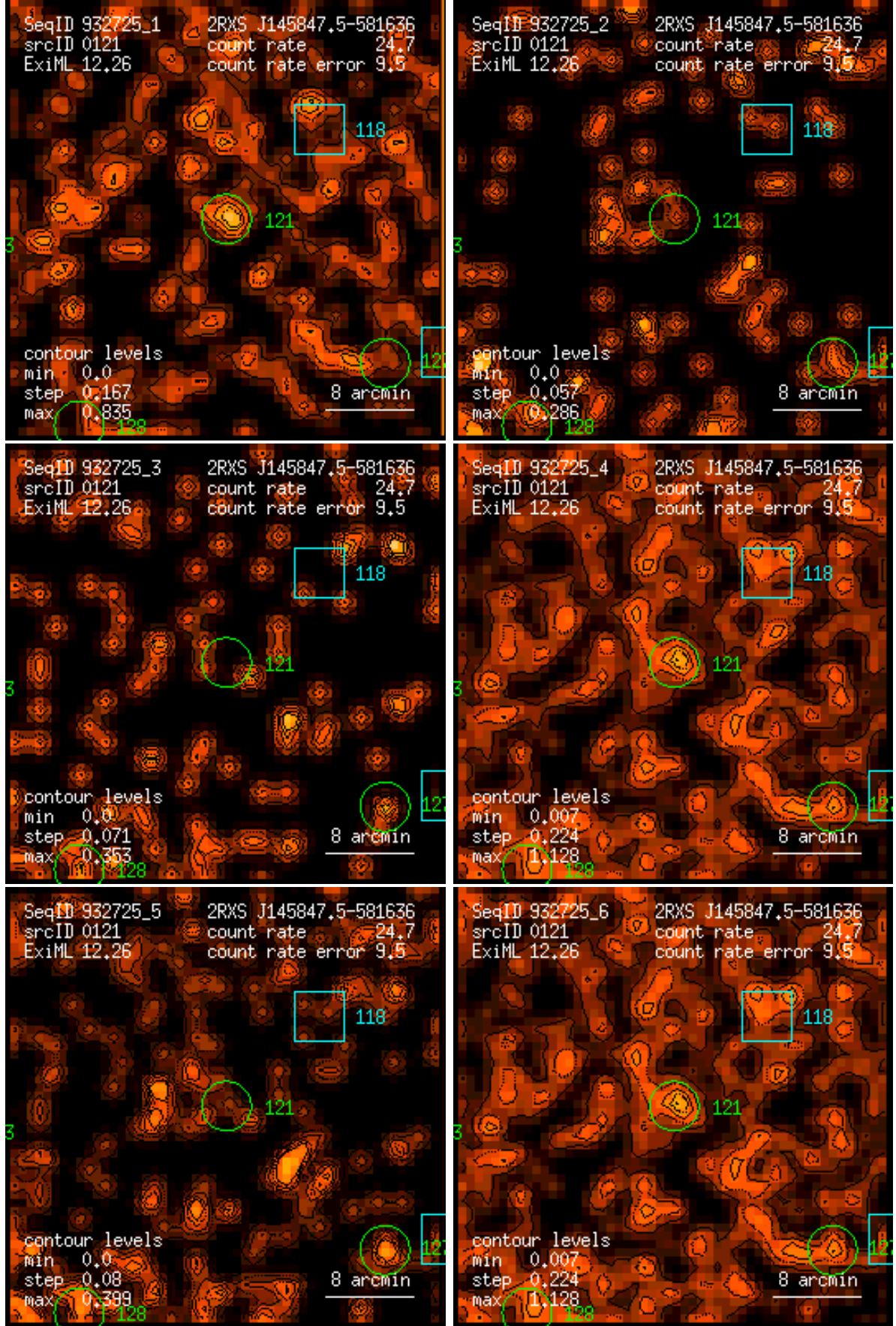
Figure 121: RASS 932725: detection 0121: band rate images, Gaussian filter: (1) PSPC channels 11 – 41, (2) 52 – 90, (3) 91 – 201, (4) 11 – 235, (5) 52 – 201, (6) 11 – 201. Broad band rates in counts/ks. Band rate contour levels in counts/ks/arcmin 2 .
