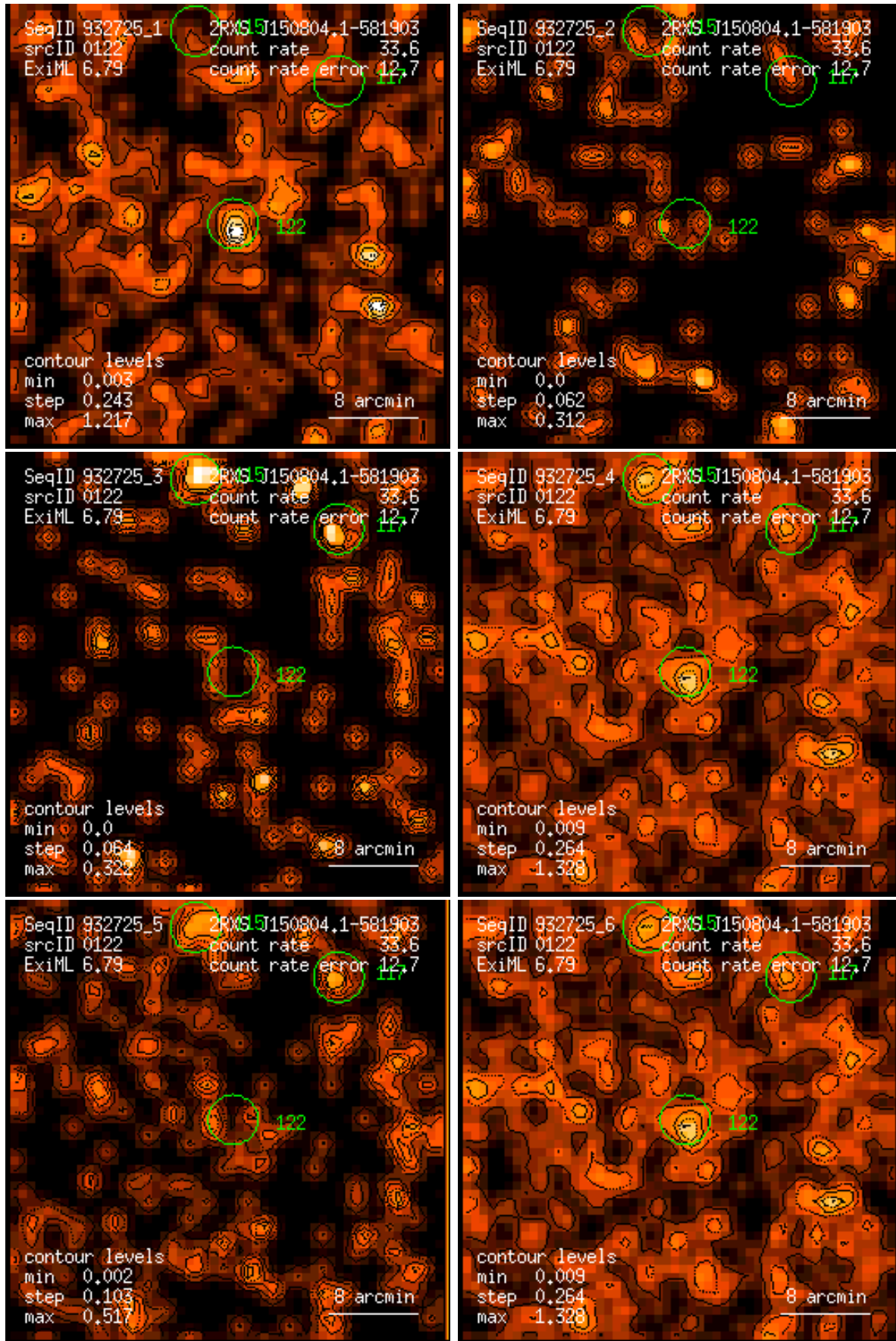
Figure 122: RASS 932725: detection 0122: band rate images, Gaussian filter: (1) PSPC channels 11 – 41, (2) 52 – 90, (3) 91 – 201, (4) 11 – 235, (5) 52 – 201, (6) 11 – 201. Broad band rates in counts/ks. Band rate contour levels in counts/ks/arcmin 2 .
