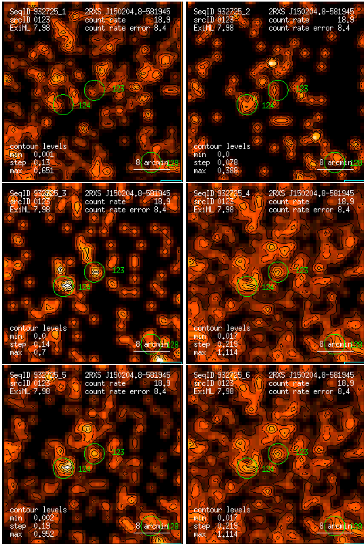
Figure 123: RASS 932725: detection 0123: band rate images, Gaussian filter: (1) PSPC channels 11 – 41, (2) 52 – 90, (3) 91 – 201, (4) 11 – 235, (5) 52 – 201, (6) 11 – 201. Broad band rates in counts/ks. Band rate contour levels in counts/ks/arcmin 2 .
