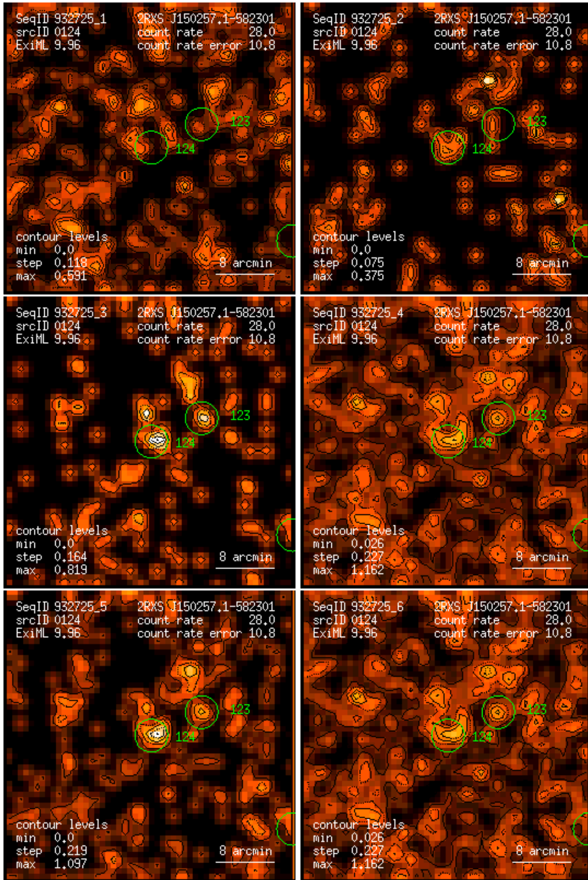
Figure 124: RASS 932725: detection 0124: band rate images, Gaussian filter: (1) PSPC channels 11 – 41, (2) 52 – 90, (3) 91 – 201, (4) 11 – 235, (5) 52 – 201, (6) 11 – 201. Broad band rates in counts/ks. Band rate contour levels in counts/ks/arcmin 2 .
