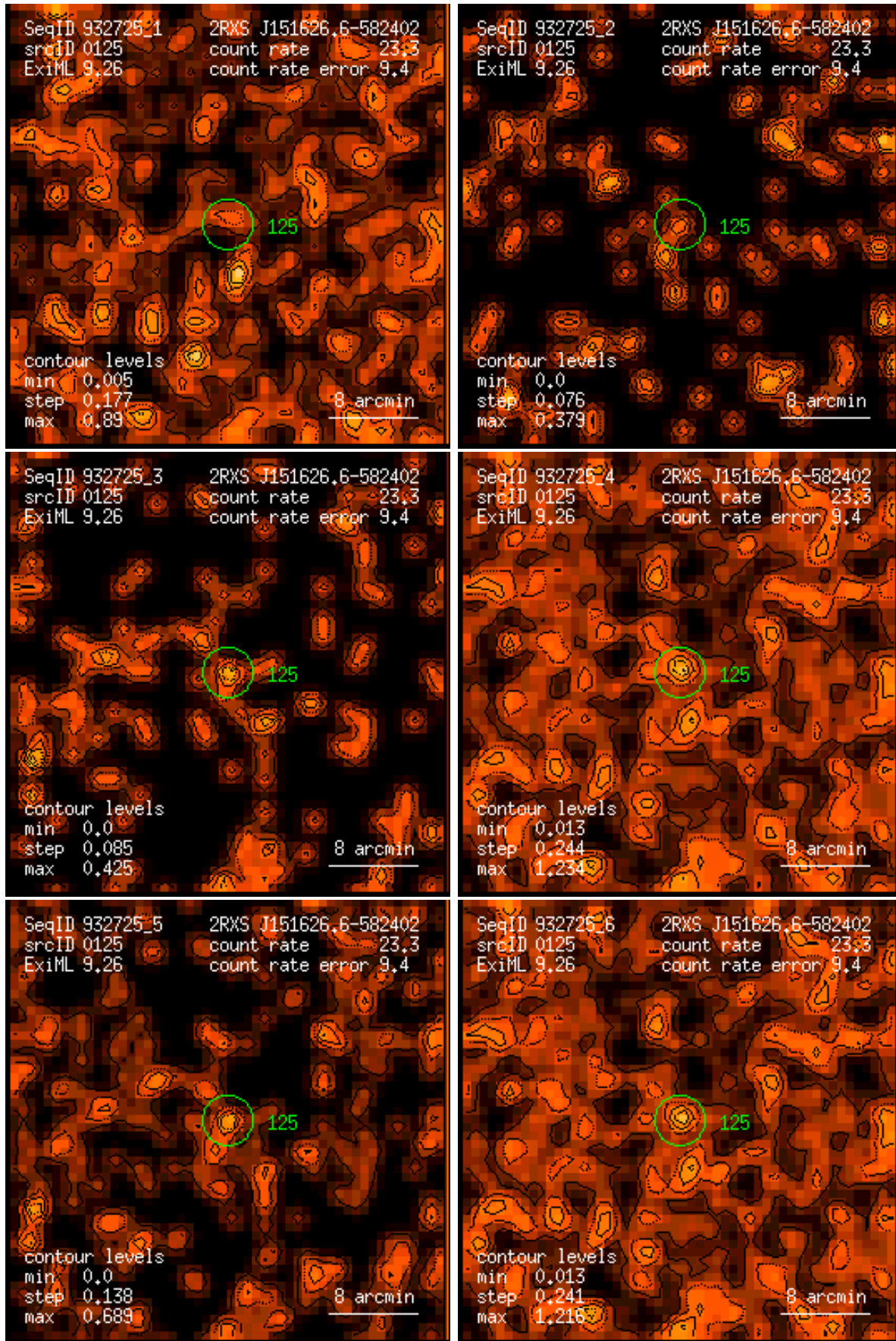
Figure 125: RASS 932725: detection 0125: band rate images, Gaussian filter: (1) PSPC channels 11 – 41, (2) 52 – 90, (3) 91 – 201, (4) 11 – 235, (5) 52 – 201, (6) 11 – 201. Broad band rates in counts/ks. Band rate contour levels in counts/ks/arcmin 2 .
