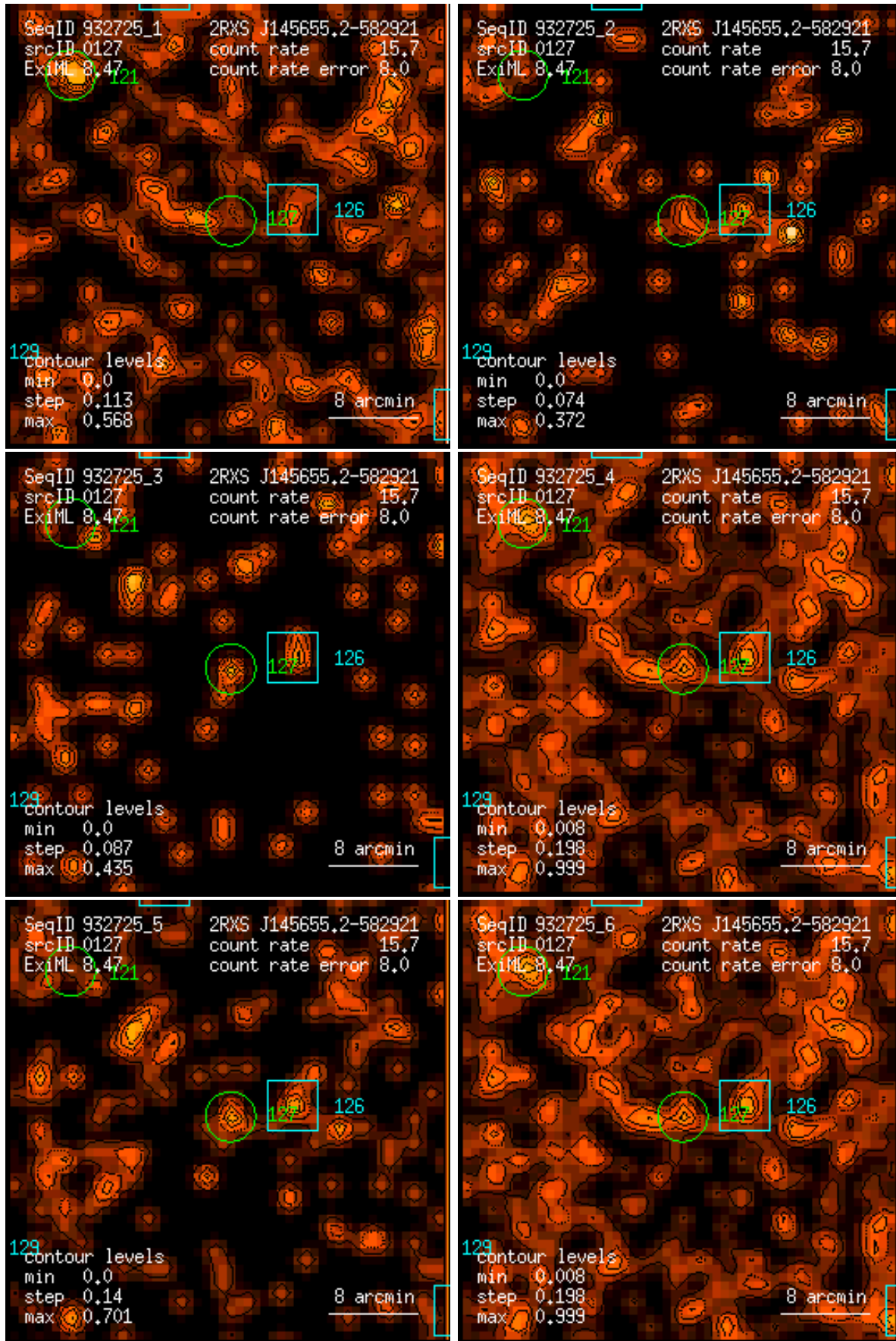
Figure 127: RASS 932725: detection 0127: band rate images, Gaussian filter: (1) PSPC channels 11 – 41, (2) 52 – 90, (3) 91 – 201, (4) 11 – 235, (5) 52 – 201, (6) 11 – 201. Broad band rates in counts/ks. Band rate contour levels in counts/ks/arcmin 2 .
