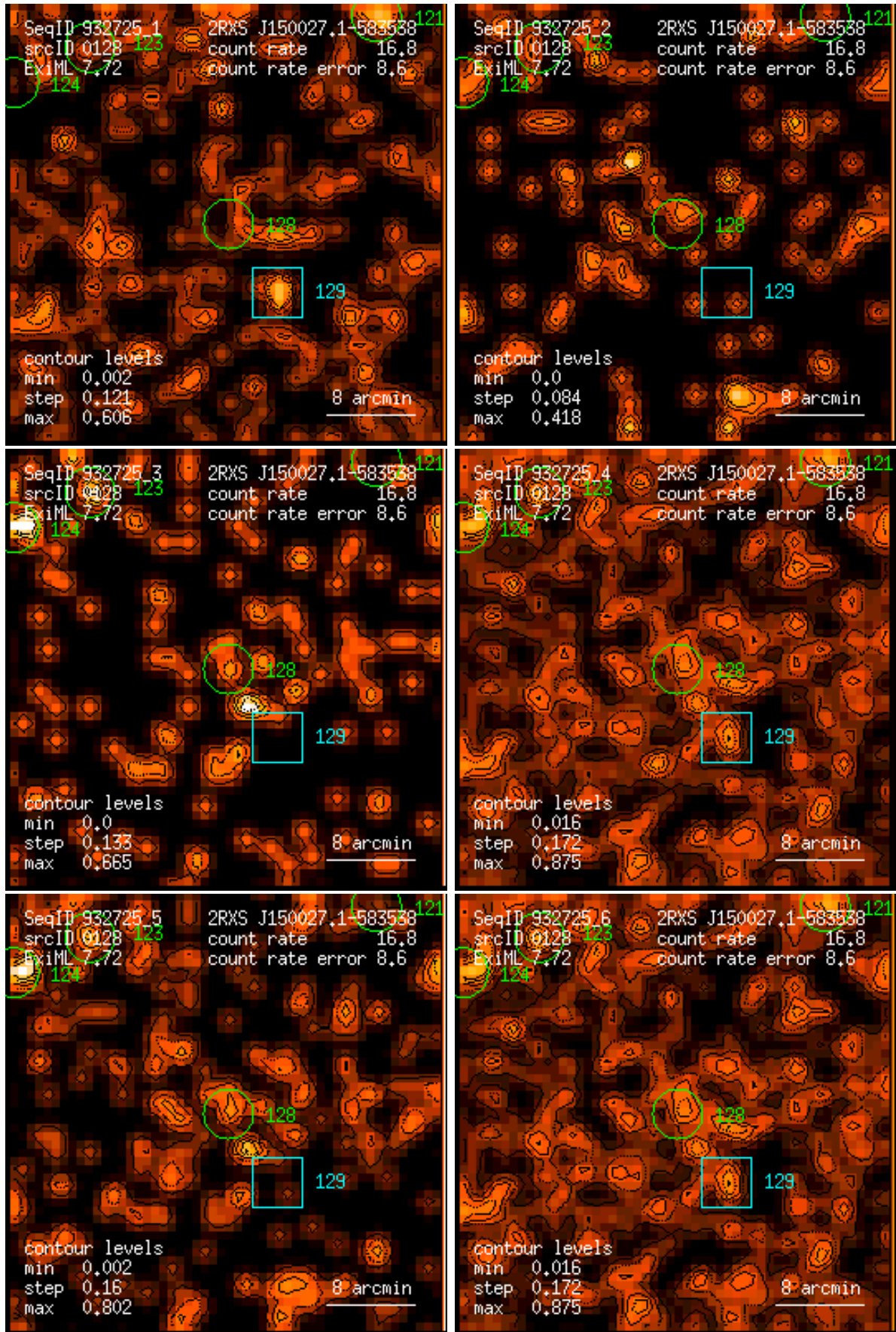
Figure 128: RASS 932725: detection 0128: band rate images, Gaussian filter: (1) PSPC channels 11 – 41, (2) 52 – 90, (3) 91 – 201, (4) 11 – 235, (5) 52 – 201, (6) 11 – 201. Broad band rates in counts/ks. Band rate contour levels in counts/ks/arcmin 2 .
