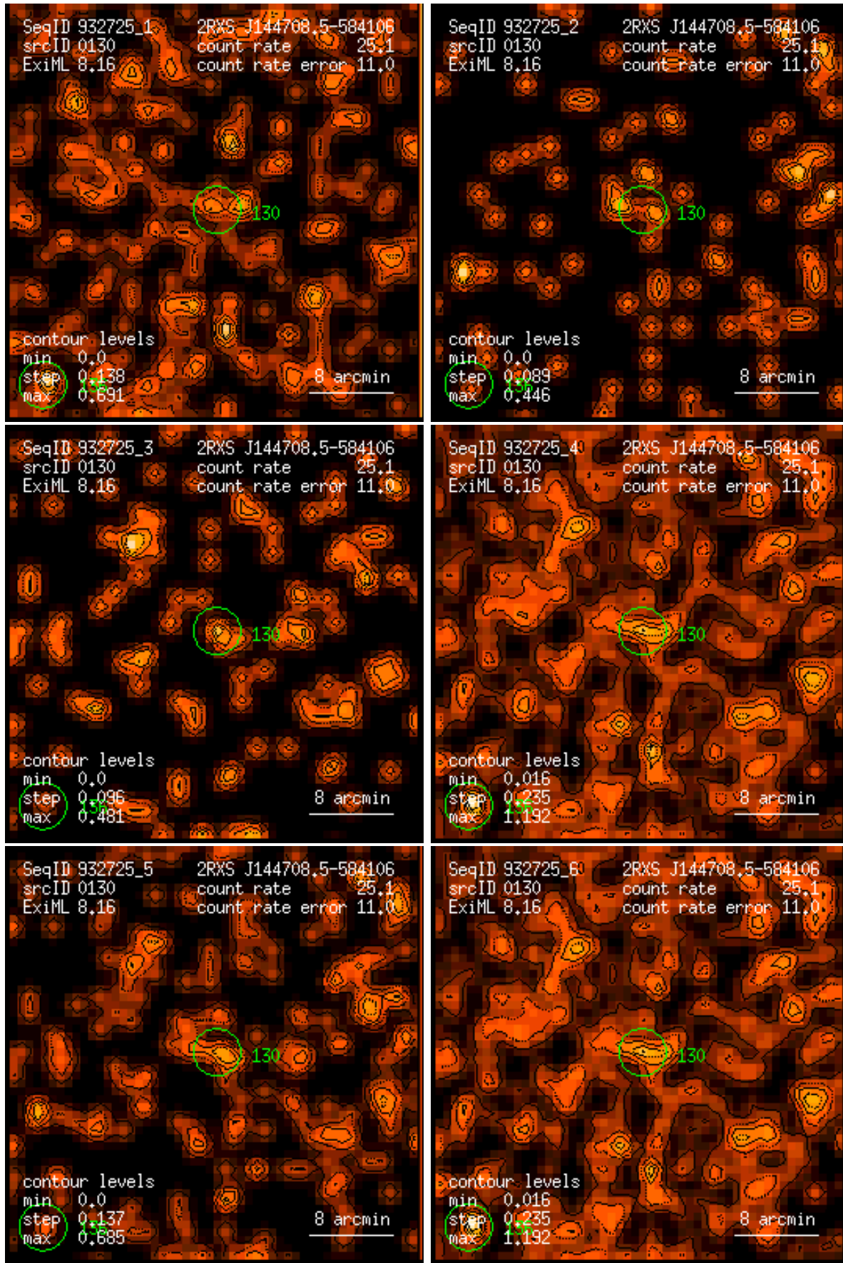
Figure 130: RASS 932725: detection 0130: band rate images, Gaussian filter: (1) PSPC channels 11 – 41, (2) 52 – 90, (3) 91 – 201, (4) 11 – 235, (5) 52 – 201, (6) 11 – 201. Broad band rates in counts/ks. Band rate contour levels in counts/ks/arcmin 2 .
