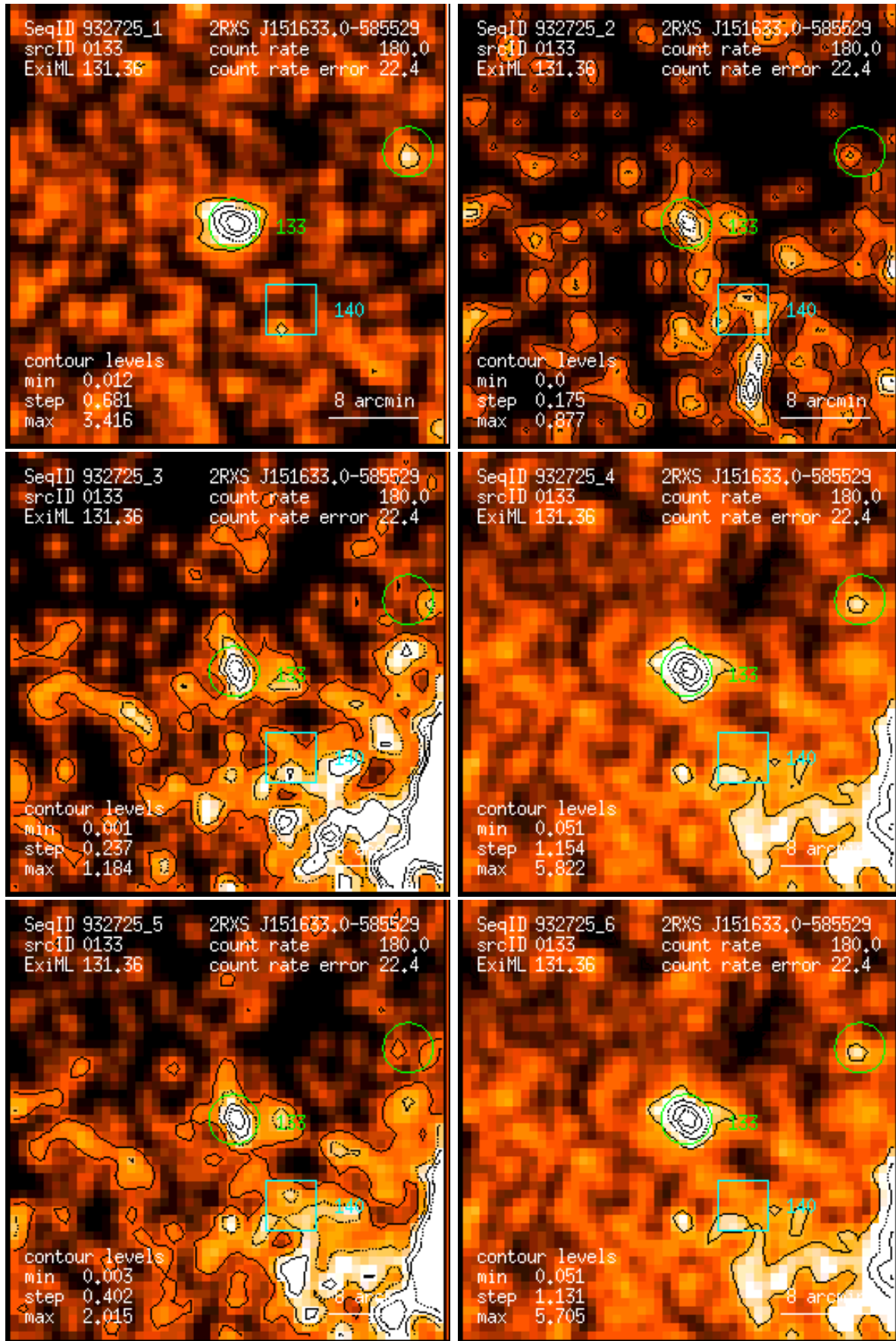
Figure 133: RASS 932725: detection 0133: band rate images, Gaussian filter: (1) PSPC channels 11 – 41, (2) 52 – 90, (3) 91 – 201, (4) 11 – 235, (5) 52 – 201, (6) 11 – 201. Broad band rates in counts/ks. Band rate contour levels in counts/ks/arcmin 2 .
