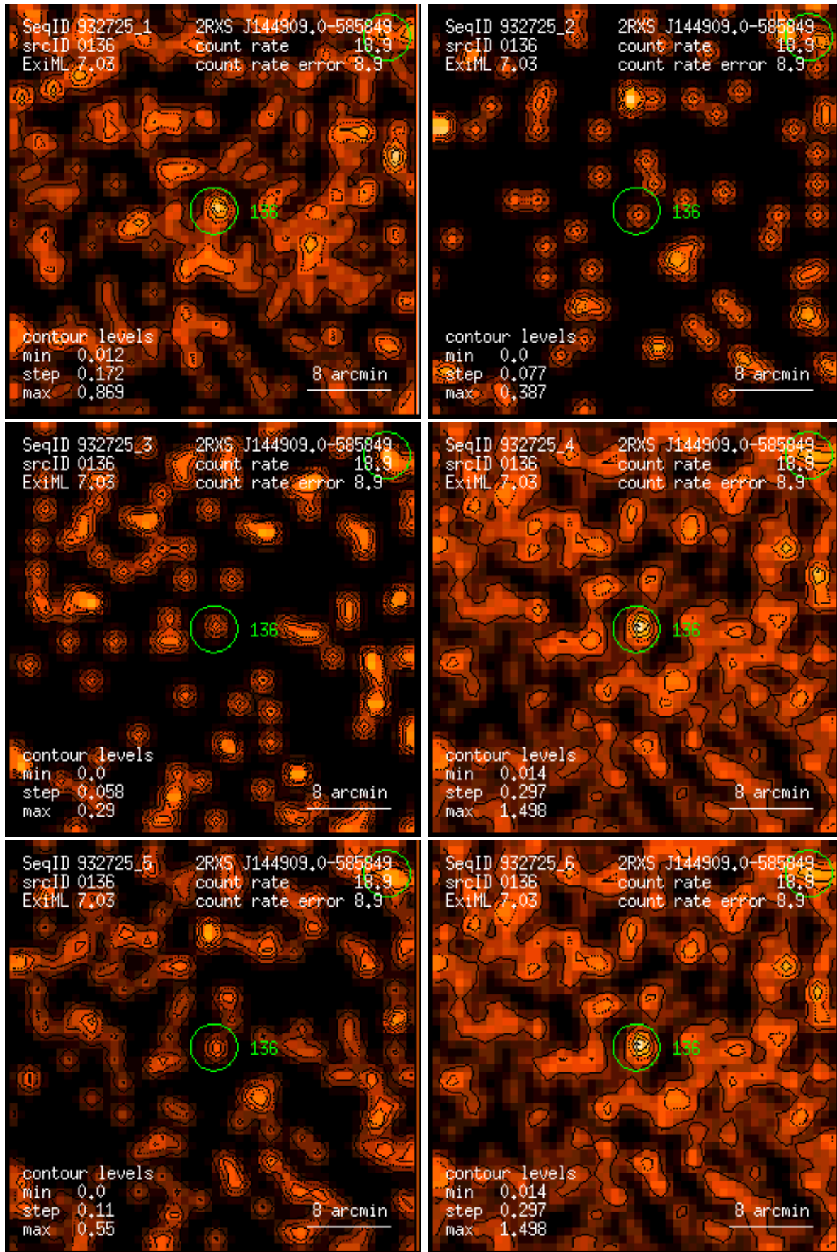
Figure 136: RASS 932725: detection 0136: band rate images, Gaussian filter: (1) PSPC channels 11 – 41, (2) 52 – 90, (3) 91 – 201, (4) 11 – 235, (5) 52 – 201, (6) 11 – 201. Broad band rates in counts/ks. Band rate contour levels in counts/ks/arcmin 2 .
