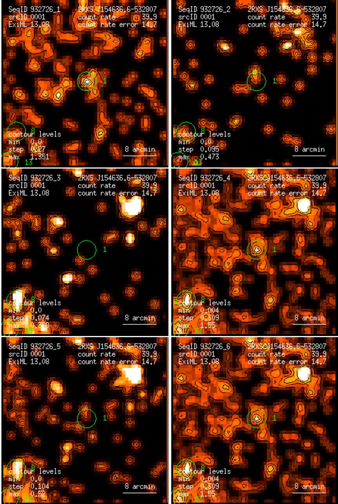
Figure 1: RASS 932726: detection 0001: band rate images, Gaussian filter: (1) PSPC channels 11 – 41, (2) 52 – 90, (3) 91 – 201, (4) 11 – 235, (5) 52 – 201, (6) 11 – 201. Broad band rates in counts/ks. Band rate contour levels in counts/ks/arcmin 2 .
