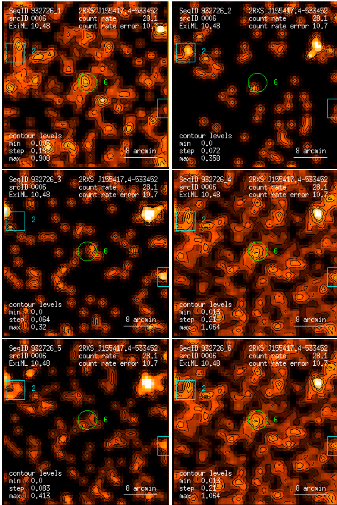
Figure 6: RASS 932726: detection 0006: band rate images, Gaussian filter: (1) PSPC channels 11 – 41, (2) 52 – 90, (3) 91 – 201, (4) 11 – 235, (5) 52 – 201, (6) 11 – 201. Broad band rates in counts/ks. Band rate contour levels in counts/ks/arcmin 2 .
