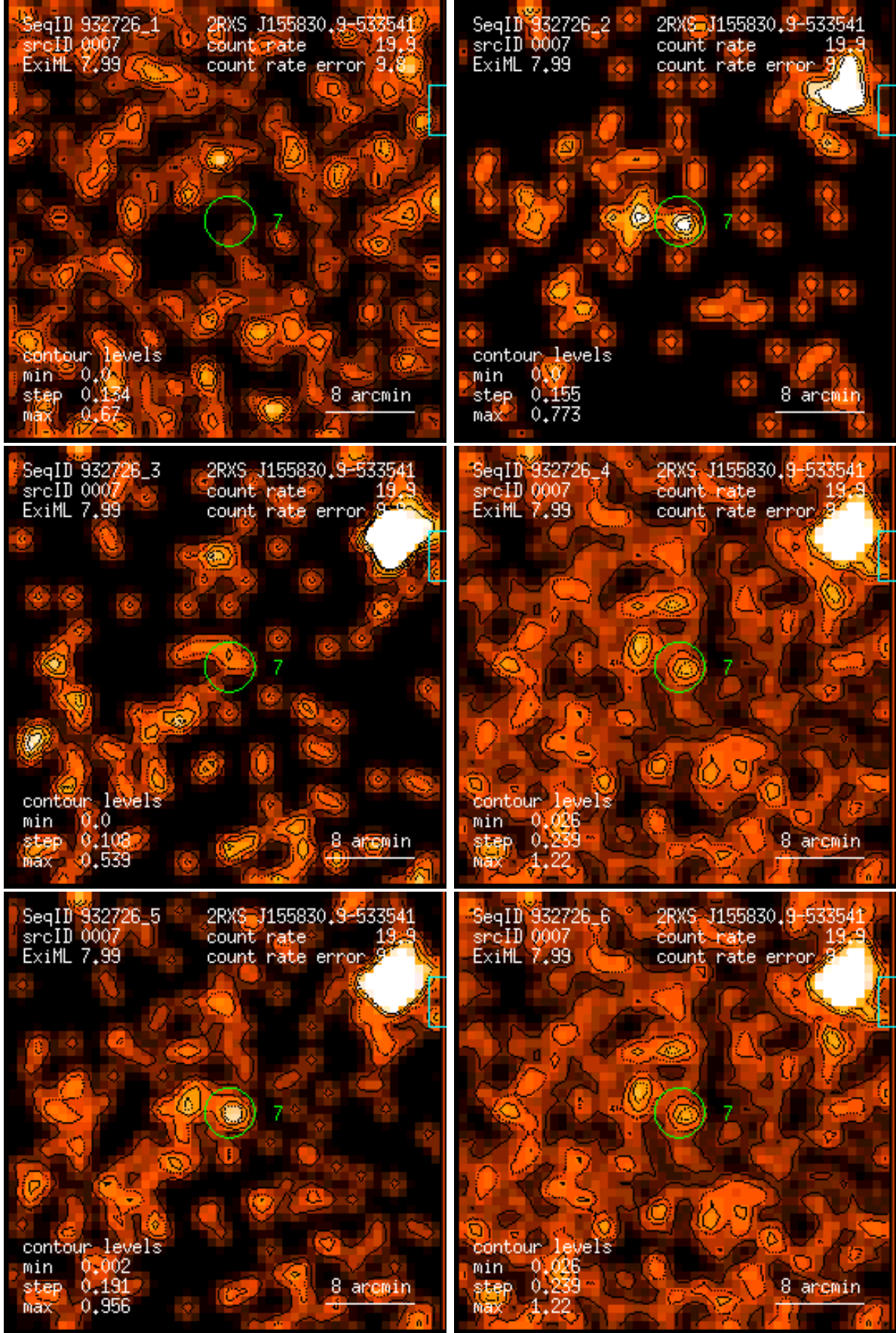
Figure 7: RASS 932726: detection 0007: band rate images, Gaussian filter: (1) PSPC channels 11 – 41, (2) 52 – 90, (3) 91 – 201, (4) 11 – 235, (5) 52 – 201, (6) 11 – 201. Broad band rates in counts/ks. Band rate contour levels in counts/ks/arcmin 2 .
