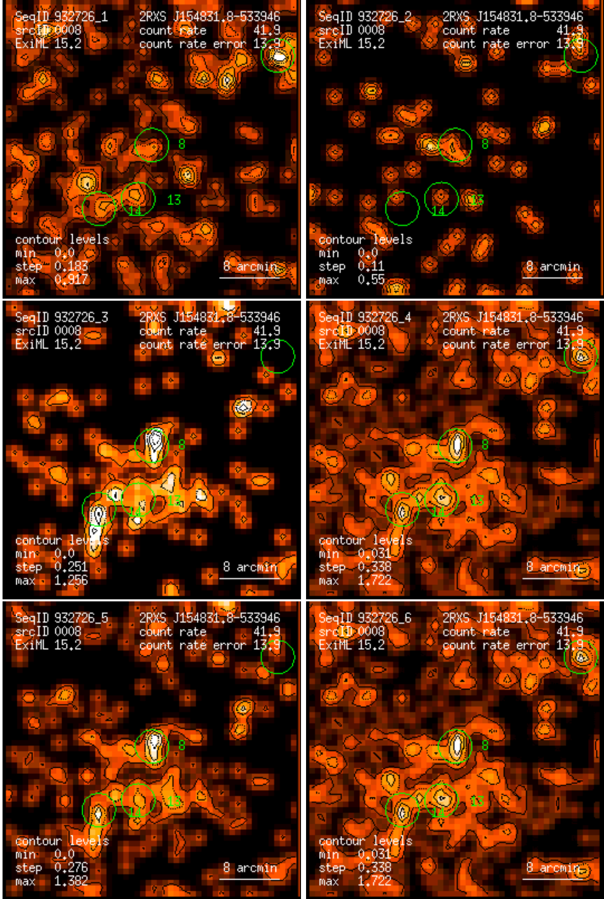
Figure 8: RASS 932726: detection 0008: band rate images, Gaussian filter: (1) PSPC channels 11 – 41, (2) 52 – 90, (3) 91 – 201, (4) 11 – 235, (5) 52 – 201, (6) 11 – 201. Broad band rates in counts/ks. Band rate contour levels in counts/ks/arcmin 2 .
