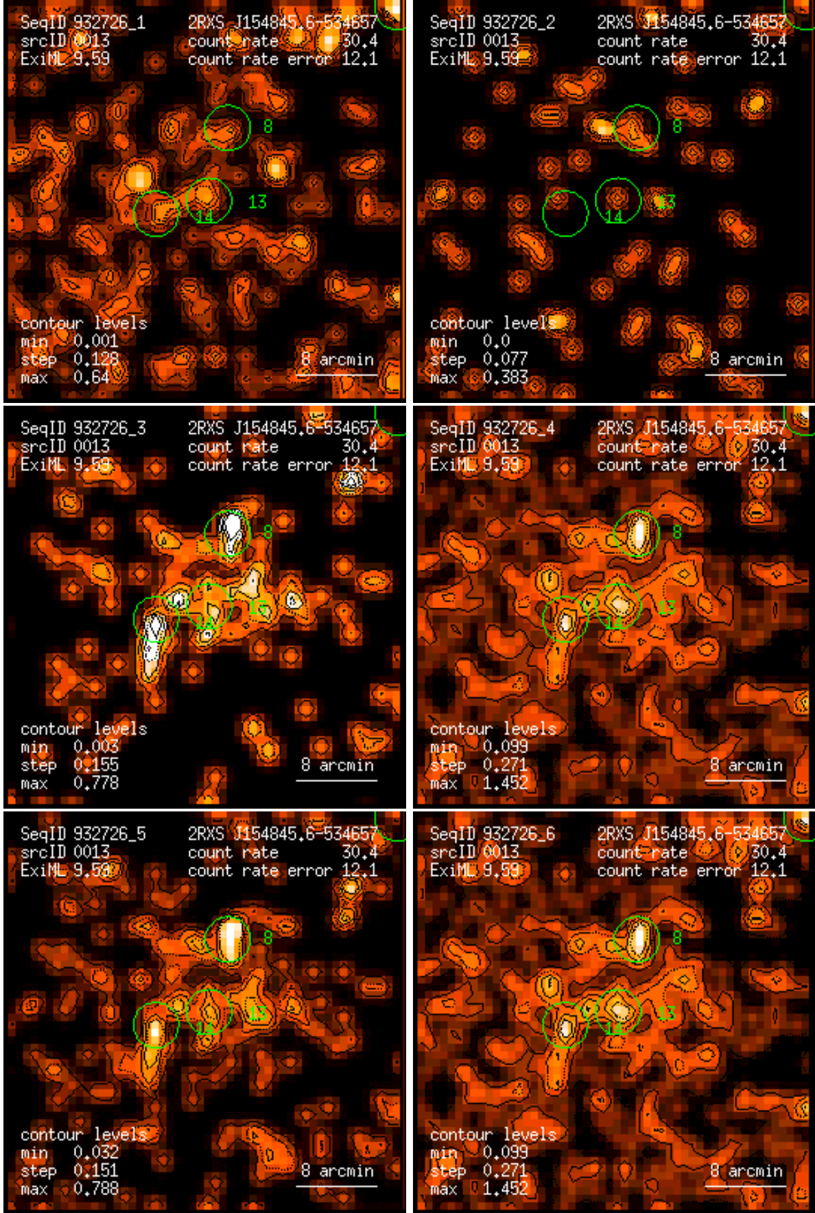
Figure 13: RASS 932726: detection 0013: band rate images, Gaussian filter: (1) PSPC channels 11 – 41, (2) 52 – 90, (3) 91 – 201, (4) 11 – 235, (5) 52 – 201, (6) 11 – 201. Broad band rates in counts/ks. Band rate contour levels in counts/ks/arcmin 2 .
