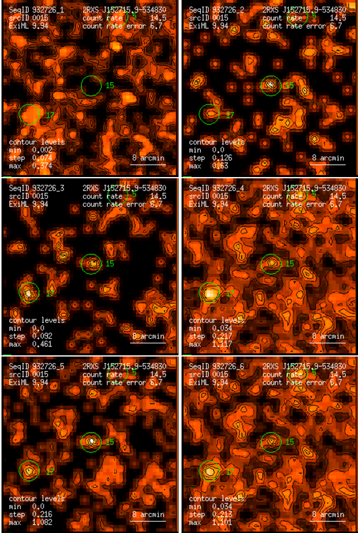
Figure 15: RASS 932726: detection 0015: band rate images, Gaussian filter: (1) PSPC channels 11 – 41, (2) 52 – 90, (3) 91 – 201, (4) 11 – 235, (5) 52 – 201, (6) 11 – 201. Broad band rates in counts/ks. Band rate contour levels in counts/ks/arcmin 2 .
