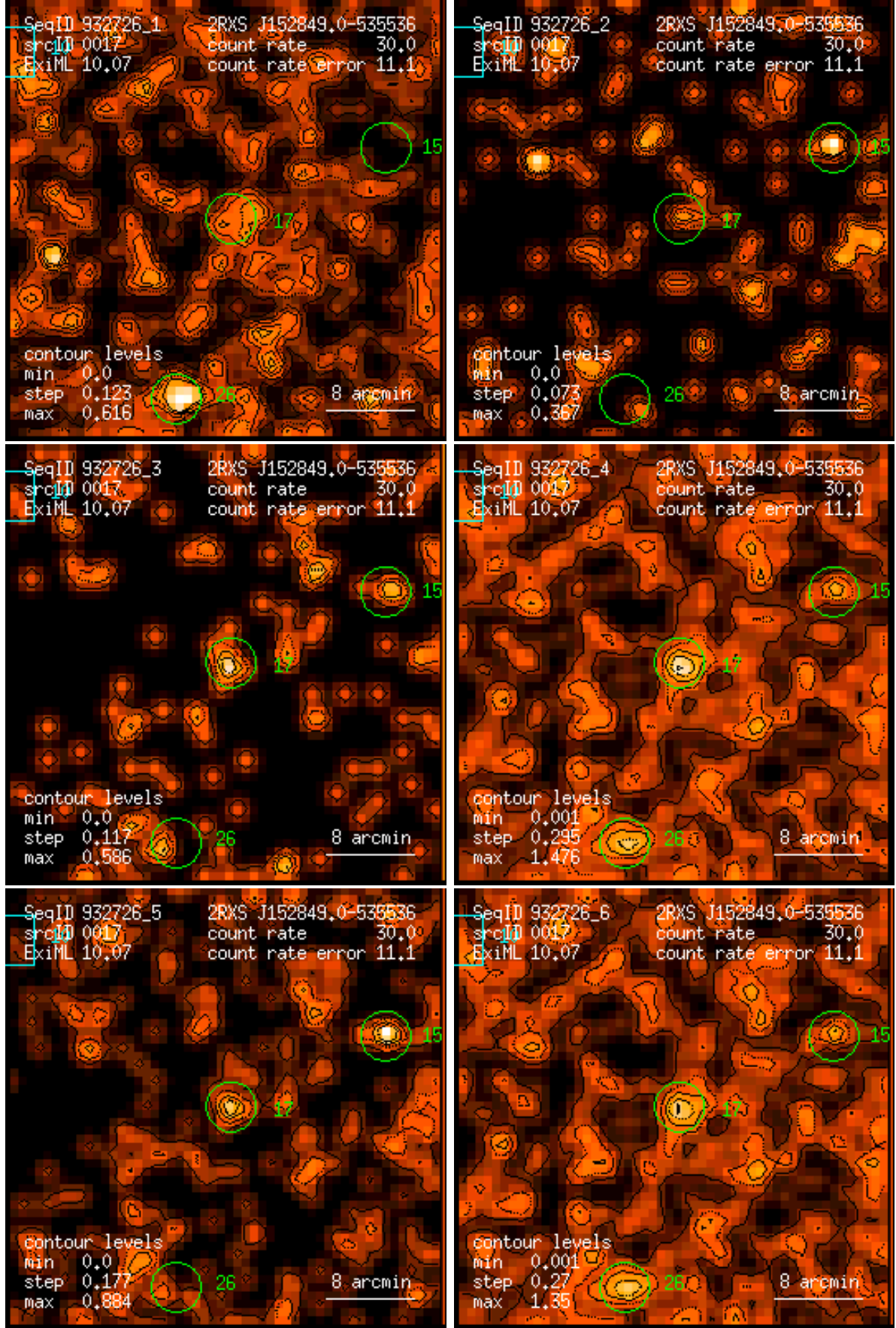
Figure 17: RASS 932726: detection 0017: band rate images, Gaussian filter: (1) PSPC channels 11 – 41, (2) 52 – 90, (3) 91 – 201, (4) 11 – 235, (5) 52 – 201, (6) 11 – 201. Broad band rates in counts/ks. Band rate contour levels in counts/ks/arcmin 2 .
