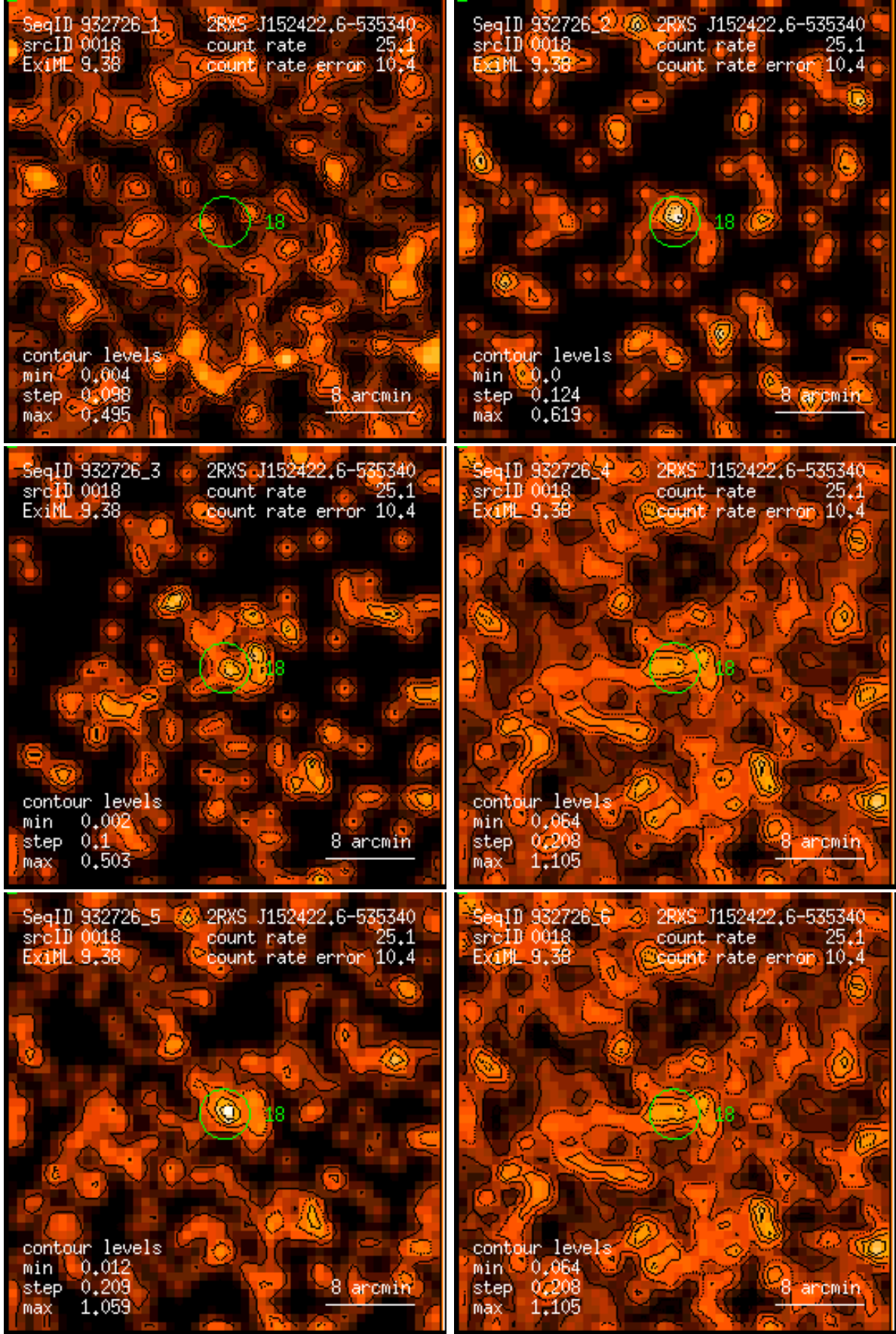
Figure 18: RASS 932726: detection 0018: band rate images, Gaussian filter: (1) PSPC channels 11 – 41, (2) 52 – 90, (3) 91 – 201, (4) 11 – 235, (5) 52 – 201, (6) 11 – 201. Broad band rates in counts/ks. Band rate contour levels in counts/ks/arcmin 2 .
