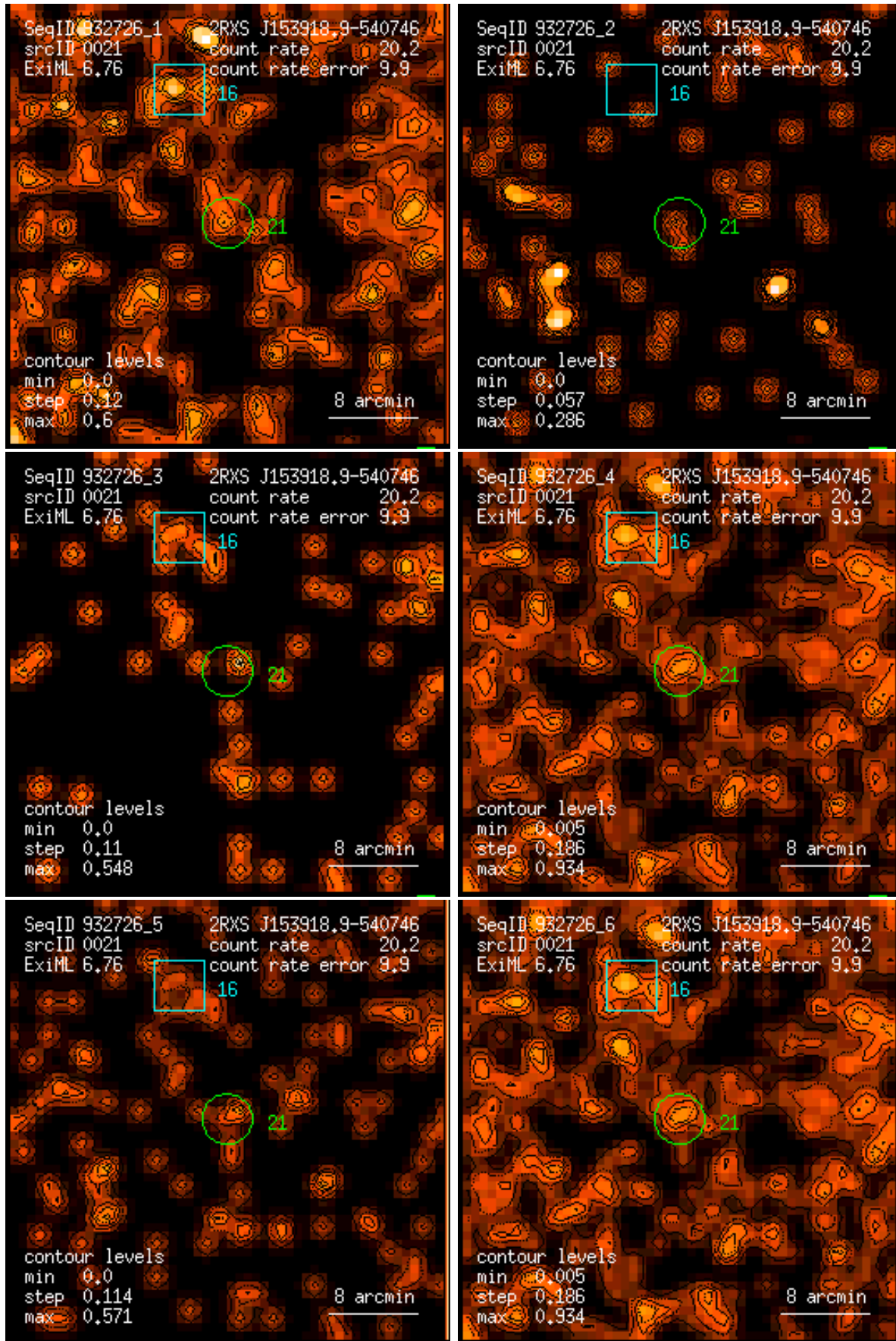
Figure 21: RASS 932726: detection 0021: band rate images, Gaussian filter: (1) PSPC channels 11 – 41, (2) 52 – 90, (3) 91 – 201, (4) 11 – 235, (5) 52 – 201, (6) 11 – 201. Broad band rates in counts/ks. Band rate contour levels in counts/ks/arcmin 2 .
