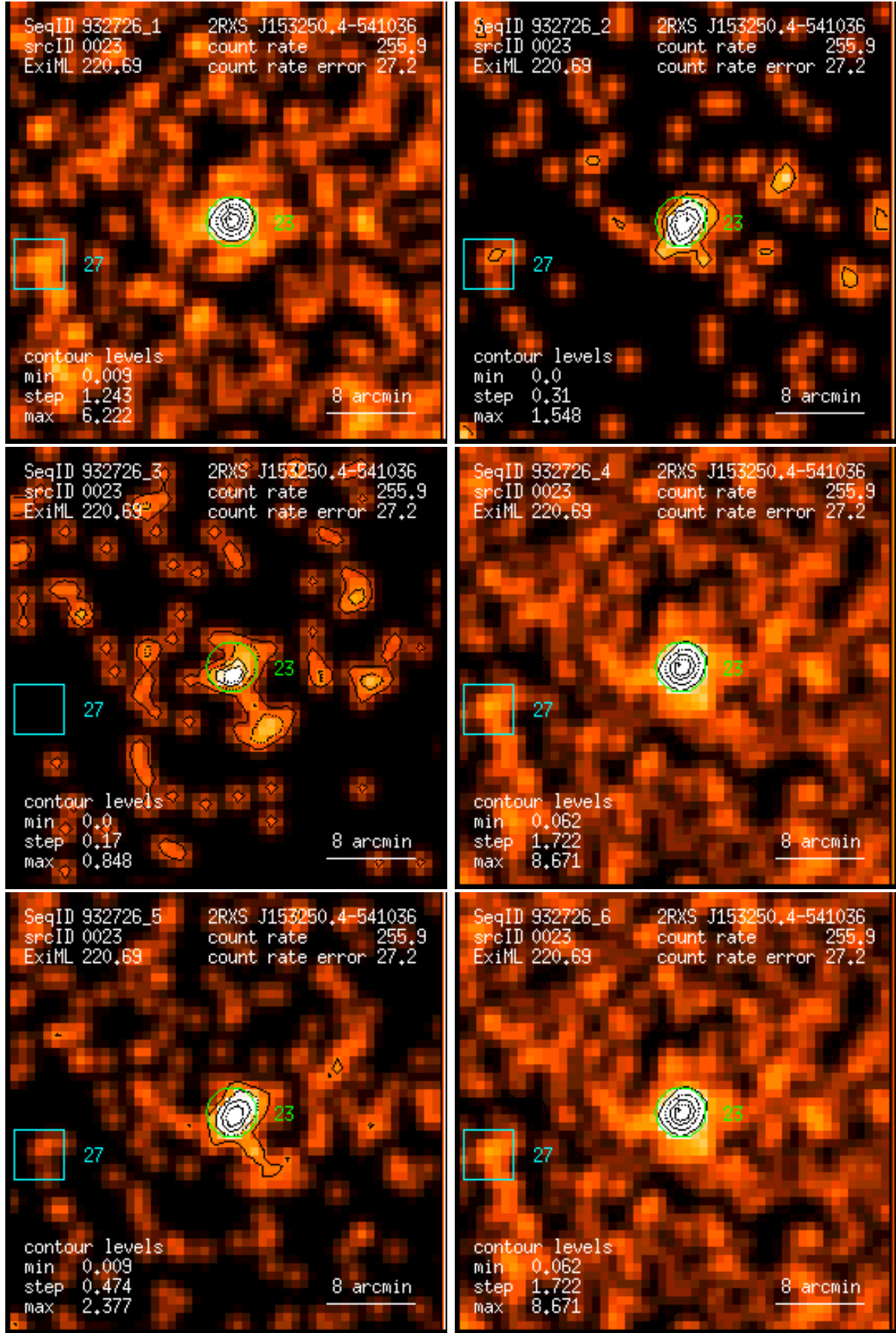
Figure 23: RASS 932726: detection 0023: band rate images, Gaussian filter: (1) PSPC channels 11 – 41, (2) 52 – 90, (3) 91 – 201, (4) 11 – 235, (5) 52 – 201, (6) 11 – 201. Broad band rates in counts/ks. Band rate contour levels in counts/ks/arcmin 2 .
