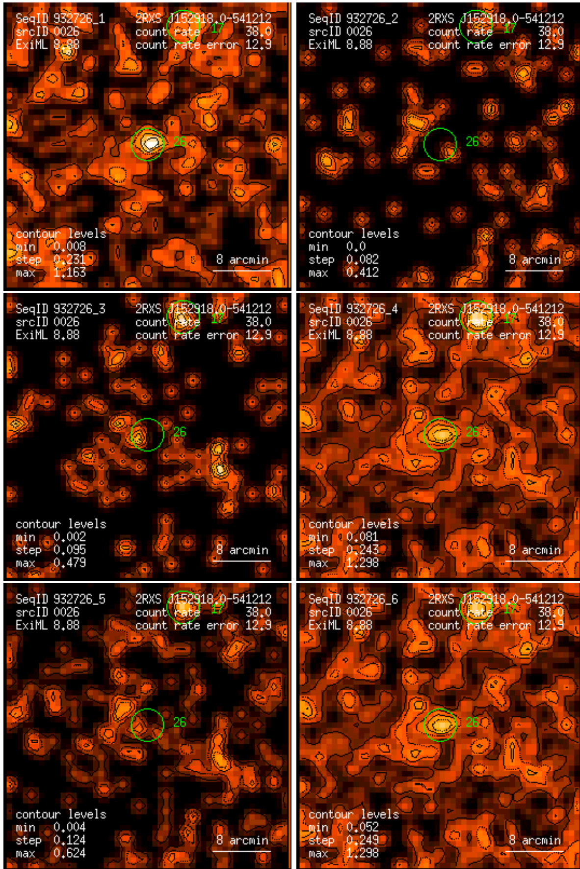
Figure 26: RASS 932726: detection 0026: band rate images, Gaussian filter: (1) PSPC channels 11 – 41, (2) 52 – 90, (3) 91 – 201, (4) 11 – 235, (5) 52 – 201, (6) 11 – 201. Broad band rates in counts/ks. Band rate contour levels in counts/ks/arcmin 2 .
