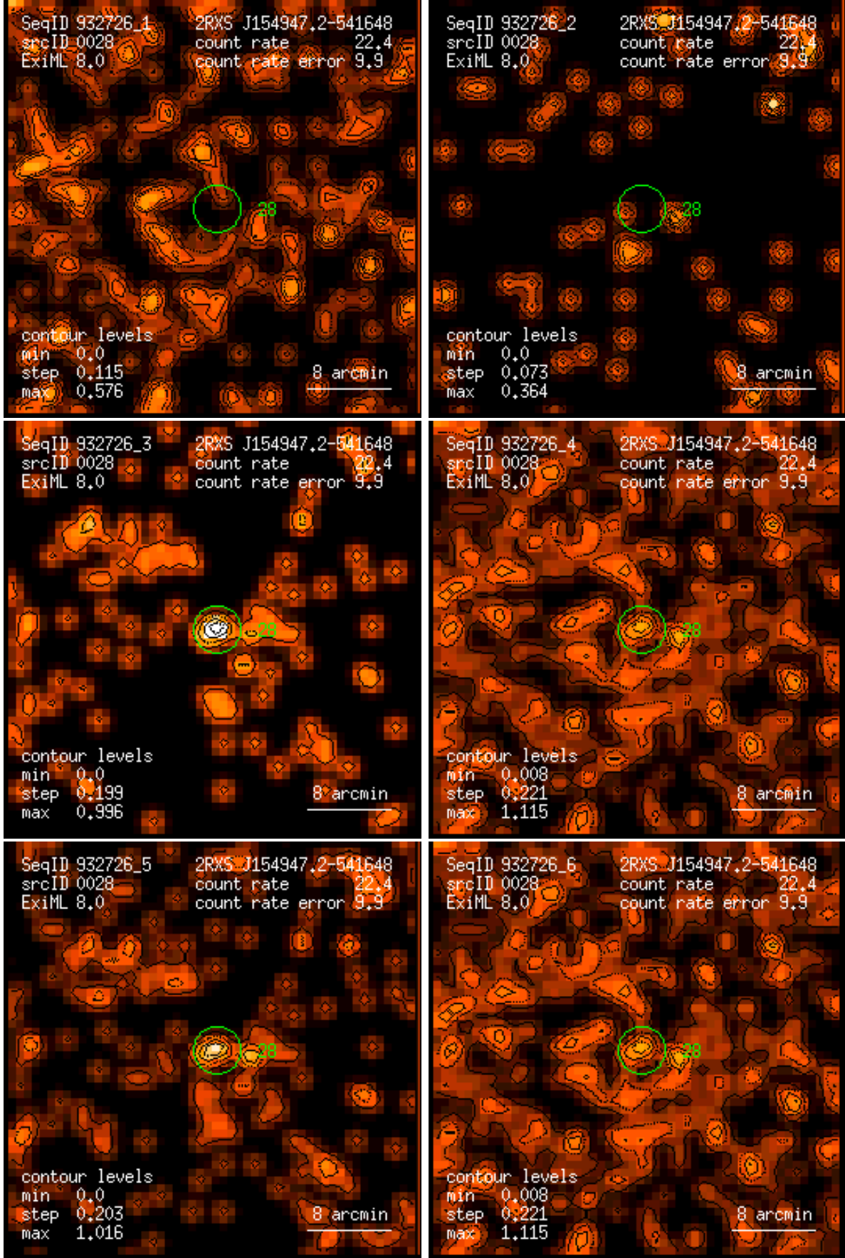
Figure 28: RASS 932726: detection 0028: band rate images, Gaussian filter: (1) PSPC channels 11 – 41, (2) 52 – 90, (3) 91 – 201, (4) 11 – 235, (5) 52 – 201, (6) 11 – 201. Broad band rates in counts/ks. Band rate contour levels in counts/ks/arcmin 2 .
