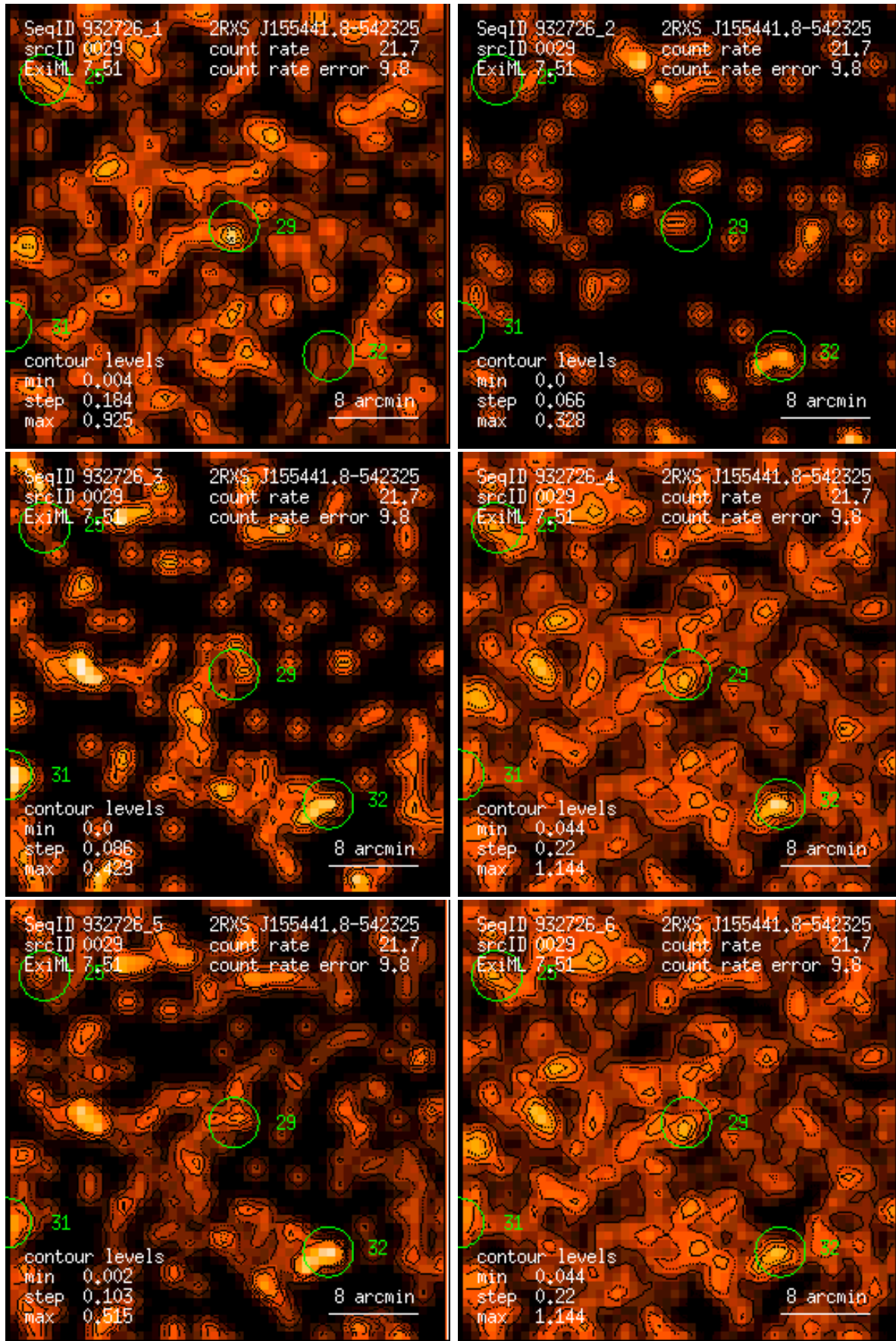
Figure 29: RASS 932726: detection 0029: band rate images, Gaussian filter: (1) PSPC channels 11 – 41, (2) 52 – 90, (3) 91 – 201, (4) 11 – 235, (5) 52 – 201, (6) 11 – 201. Broad band rates in counts/ks. Band rate contour levels in counts/ks/arcmin 2 .
