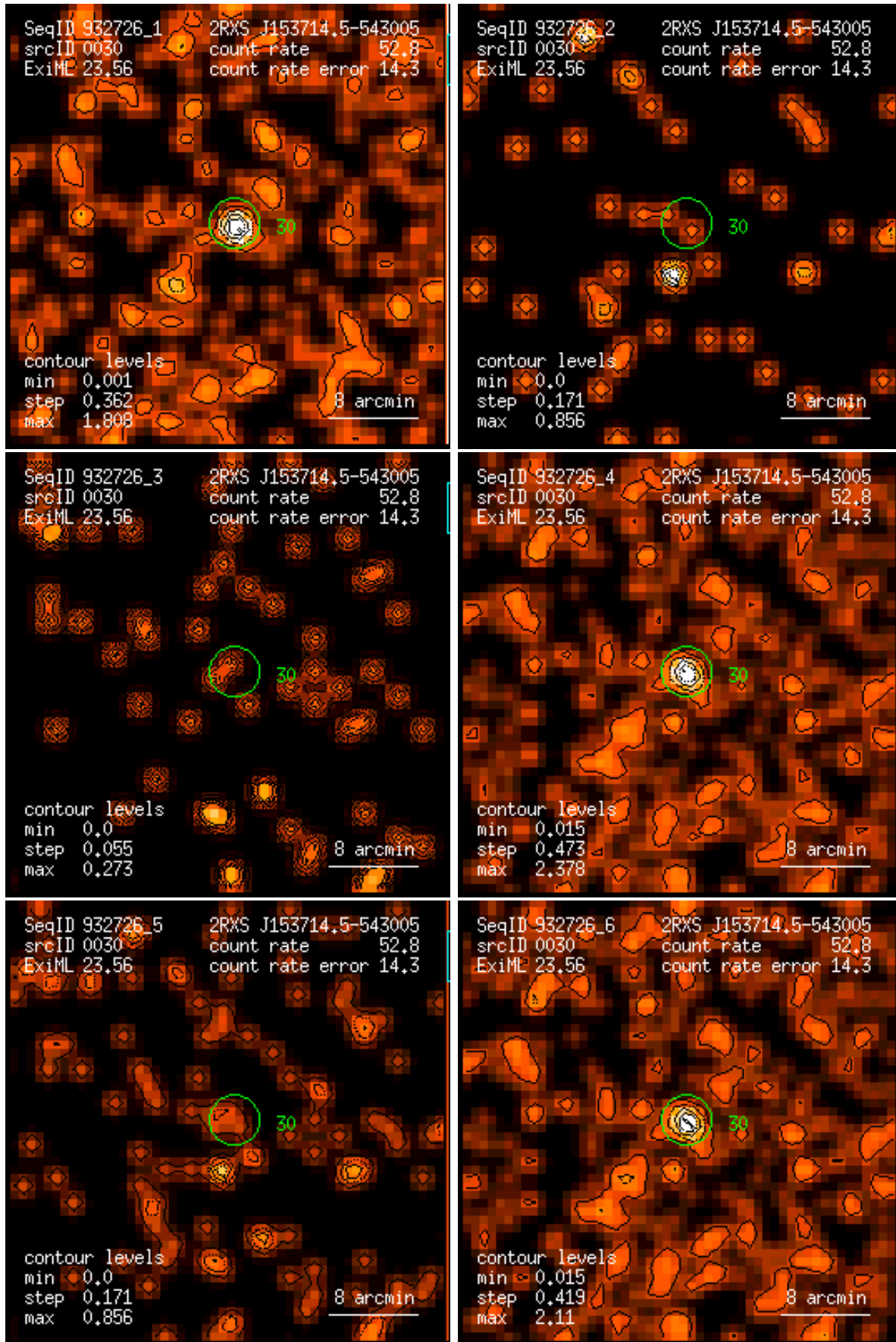
Figure 30: RASS 932726: detection 0030: band rate images, Gaussian filter: (1) PSPC channels 11 – 41, (2) 52 – 90, (3) 91 – 201, (4) 11 – 235, (5) 52 – 201, (6) 11 – 201. Broad band rates in counts/ks. Band rate contour levels in counts/ks/arcmin 2 .
