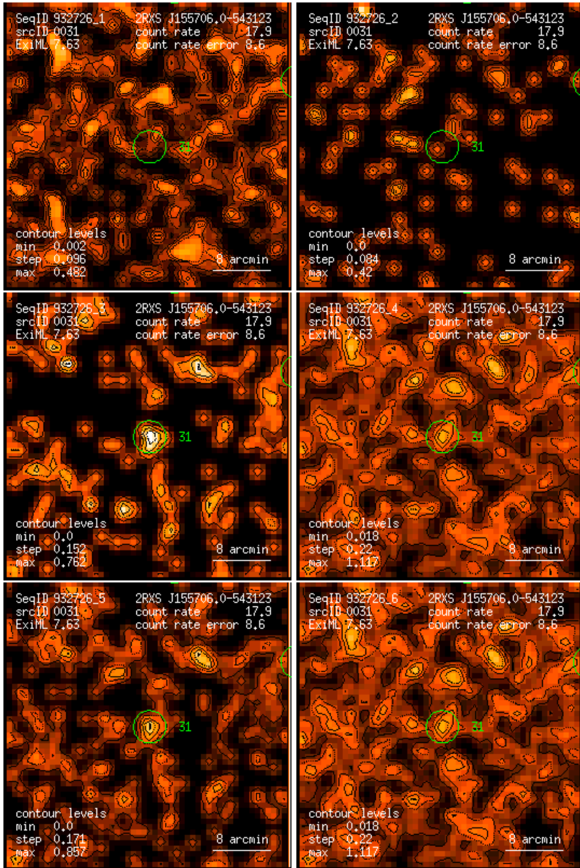
Figure 31: RASS 932726: detection 0031: band rate images, Gaussian filter: (1) PSPC channels 11 – 41, (2) 52 – 90, (3) 91 – 201, (4) 11 – 235, (5) 52 – 201, (6) 11 – 201. Broad band rates in counts/ks. Band rate contour levels in counts/ks/arcmin 2 .
