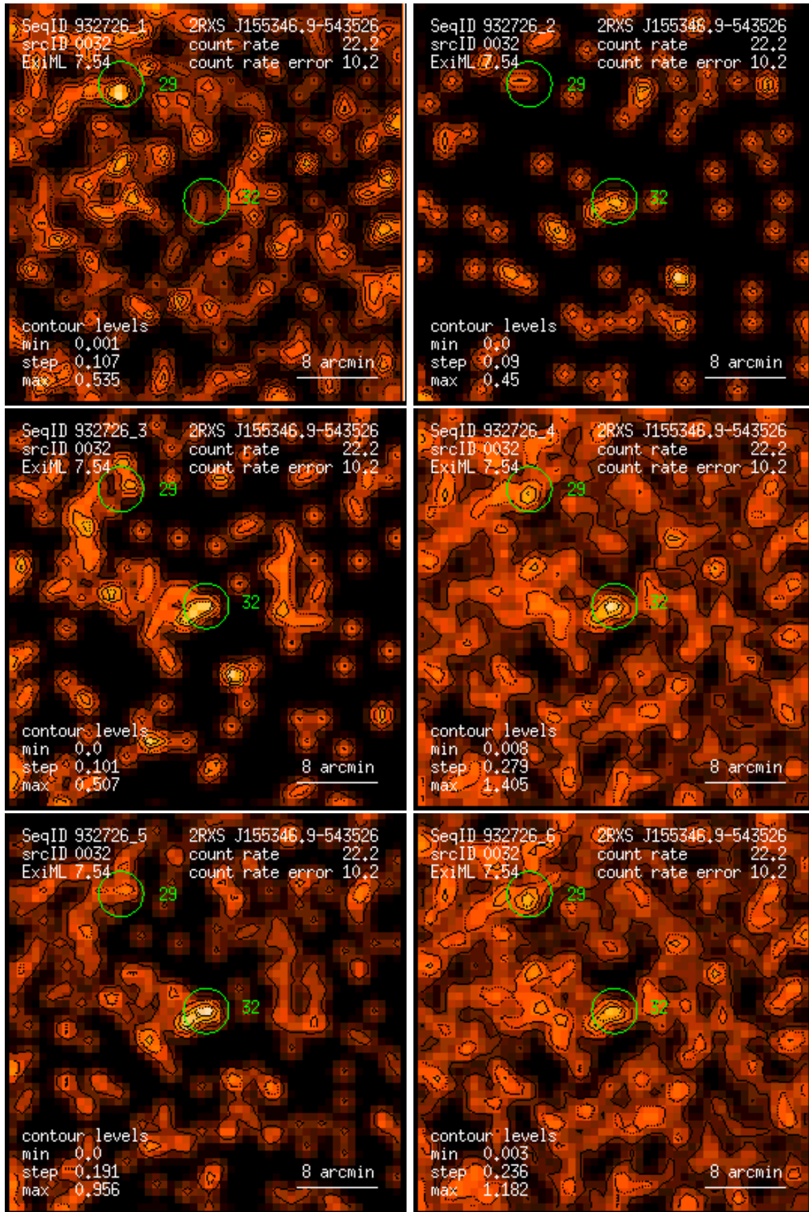
Figure 32: RASS 932726: detection 0032: band rate images, Gaussian filter: (1) PSPC channels 11 – 41, (2) 52 – 90, (3) 91 – 201, (4) 11 – 235, (5) 52 – 201, (6) 11 – 201. Broad band rates in counts/ks. Band rate contour levels in counts/ks/arcmin 2 .
