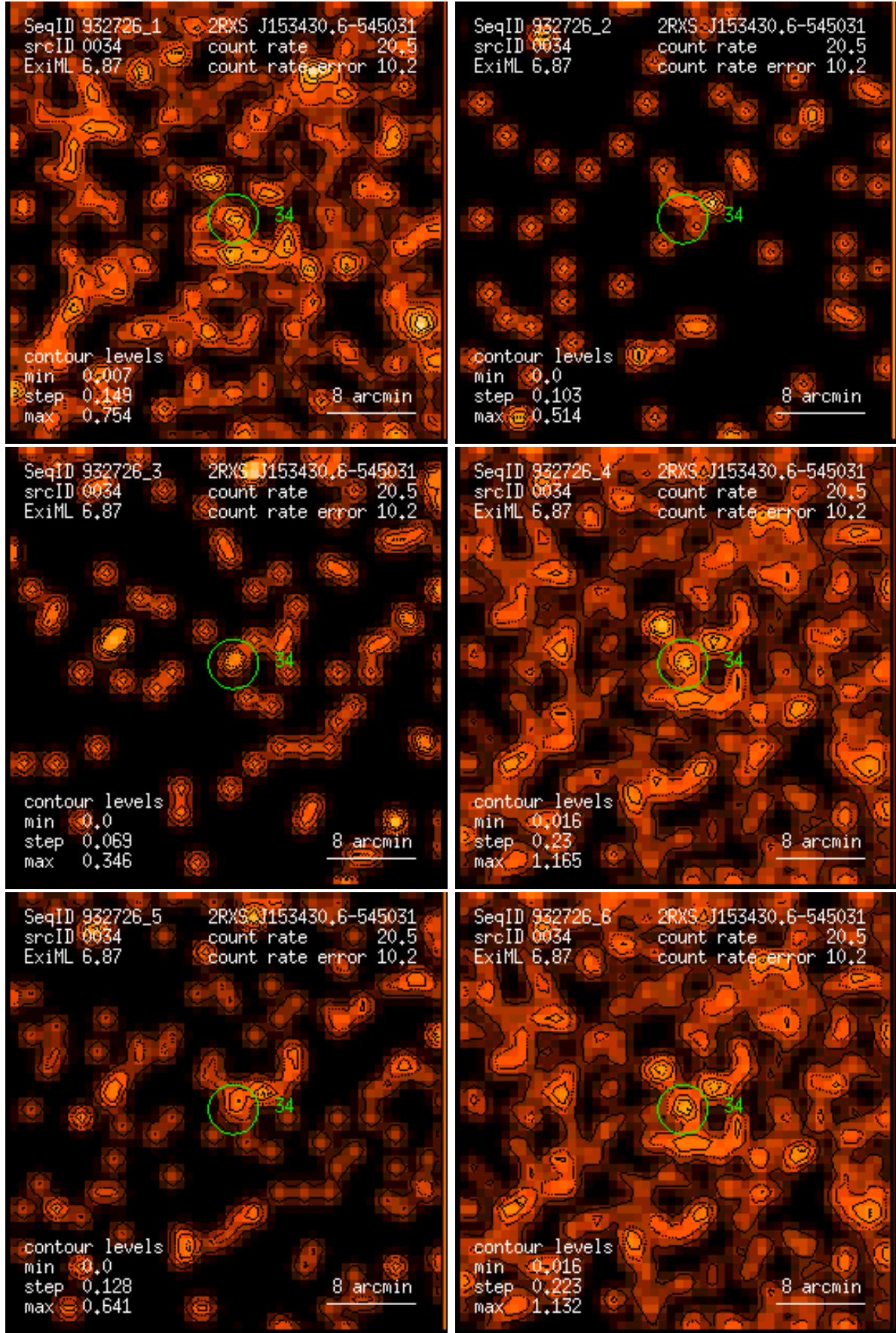
Figure 34: RASS 932726: detection 0034: band rate images, Gaussian filter: (1) PSPC channels 11 – 41, (2) 52 – 90, (3) 91 – 201, (4) 11 – 235, (5) 52 – 201, (6) 11 – 201. Broad band rates in counts/ks. Band rate contour levels in counts/ks/arcmin 2 .
