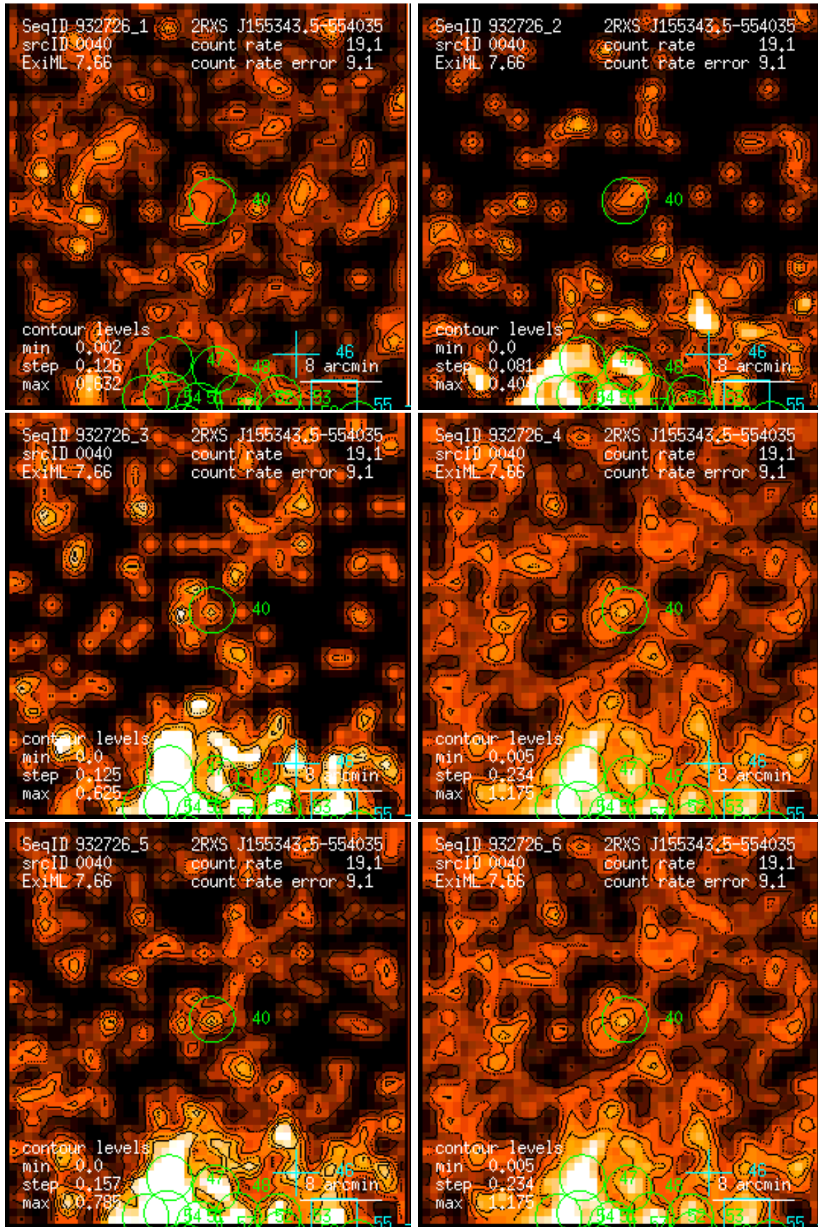
Figure 40: RASS 932726: detection 0040: band rate images, Gaussian filter: (1) PSPC channels 11 – 41, (2) 52 – 90, (3) 91 – 201, (4) 11 – 235, (5) 52 – 201, (6) 11 – 201. Broad band rates in counts/ks. Band rate contour levels in counts/ks/arcmin 2 .
