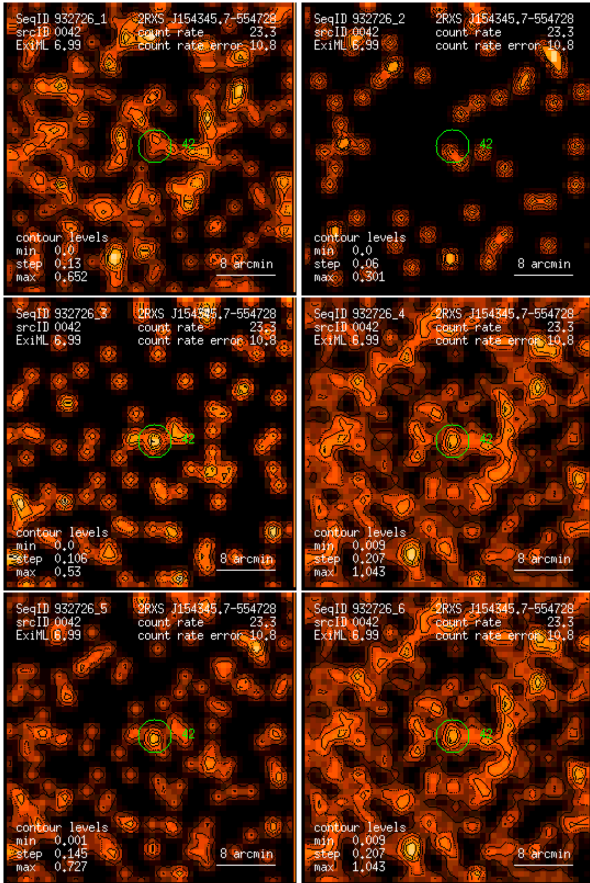
Figure 42: RASS 932726: detection 0042: band rate images, Gaussian filter: (1) PSPC channels 11 – 41, (2) 52 – 90, (3) 91 – 201, (4) 11 – 235, (5) 52 – 201, (6) 11 – 201. Broad band rates in counts/ks. Band rate contour levels in counts/ks/arcmin 2 .
