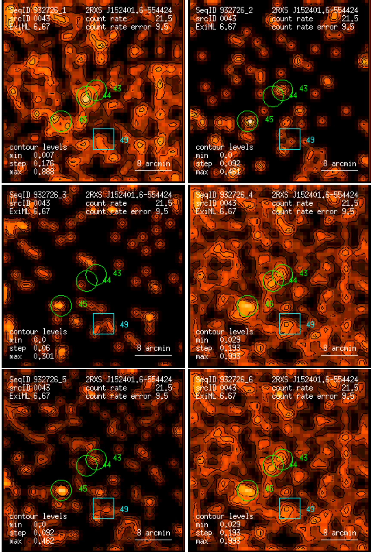
Figure 43: RASS 932726: detection 0043: band rate images, Gaussian filter: (1) PSPC channels 11 – 41, (2) 52 – 90, (3) 91 – 201, (4) 11 – 235, (5) 52 – 201, (6) 11 – 201. Broad band rates in counts/ks. Band rate contour levels in counts/ks/arcmin 2 .
