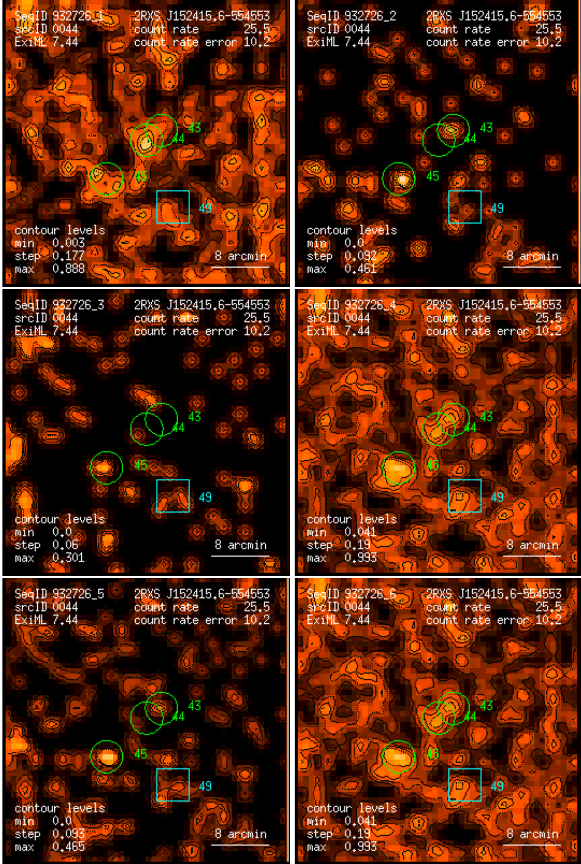
Figure 44: RASS 932726: detection 0044: band rate images, Gaussian filter: (1) PSPC channels 11 – 41, (2) 52 – 90, (3) 91 – 201, (4) 11 – 235, (5) 52 – 201, (6) 11 – 201. Broad band rates in counts/ks. Band rate contour levels in counts/ks/arcmin 2 .
