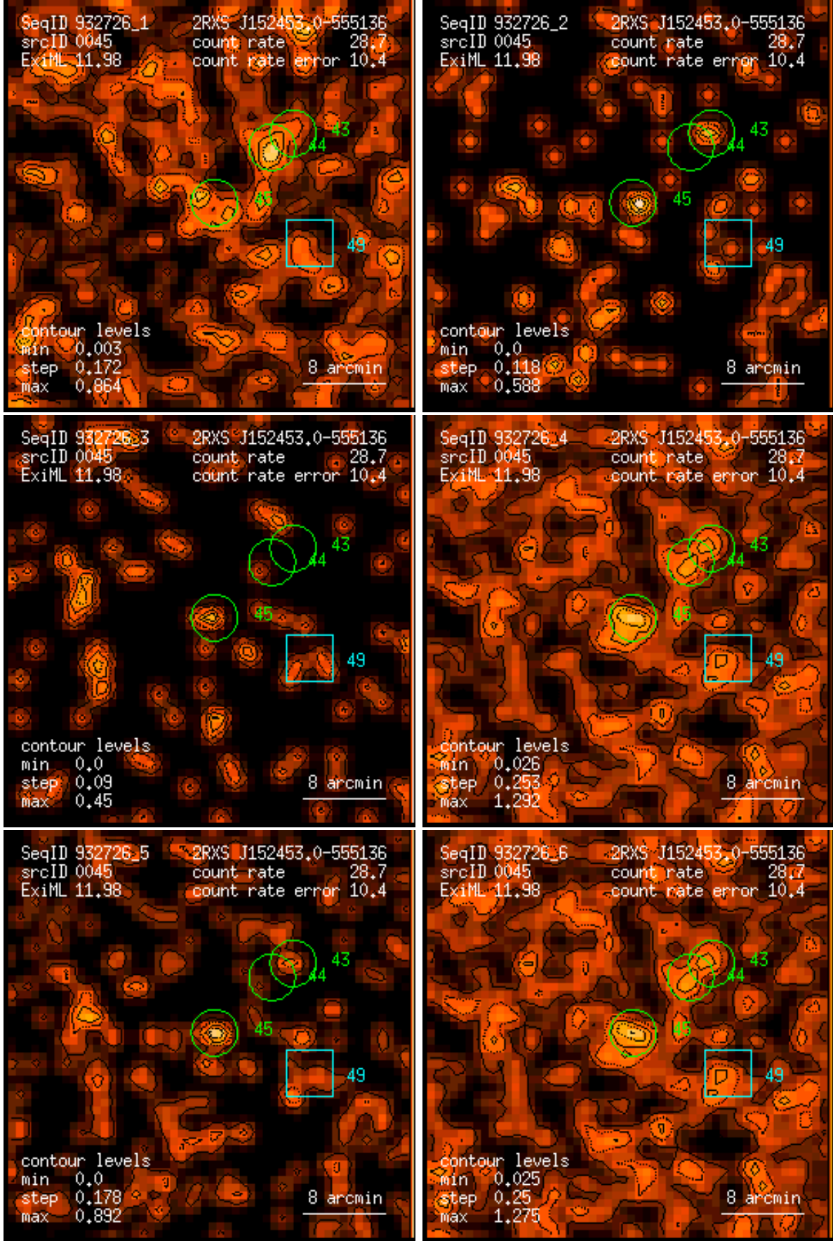
Figure 45: RASS 932726: detection 0045: band rate images, Gaussian filter: (1) PSPC channels 11 – 41, (2) 52 – 90, (3) 91 – 201, (4) 11 – 235, (5) 52 – 201, (6) 11 – 201. Broad band rates in counts/ks. Band rate contour levels in counts/ks/arcmin 2 .
