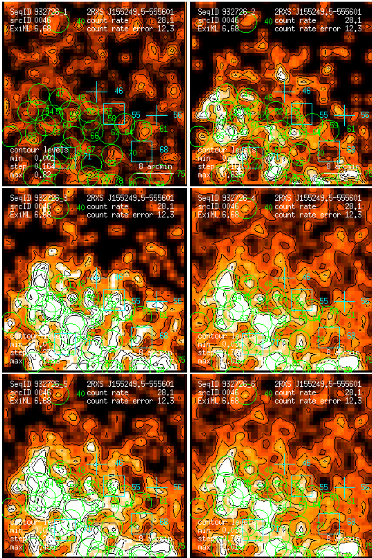
Figure 46: RASS 932726: detection 0046: band rate images, Gaussian filter: (1) PSPC channels 11 – 41, (2) 52 – 90, (3) 91 – 201, (4) 11 – 235, (5) 52 – 201, (6) 11 – 201. Broad band rates in counts/ks. Band rate contour levels in counts/ks/arcmin 2 .
