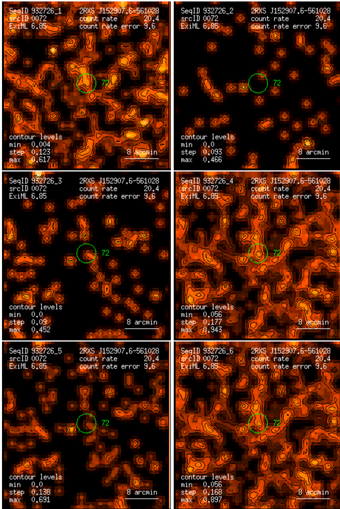
Figure 72: RASS 932726: detection 0072: band rate images, Gaussian filter: (1) PSPC channels 11 – 41, (2) 52 – 90, (3) 91 – 201, (4) 11 – 235, (5) 52 – 201, (6) 11 – 201. Broad band rates in counts/ks. Band rate contour levels in counts/ks/arcmin 2 .
