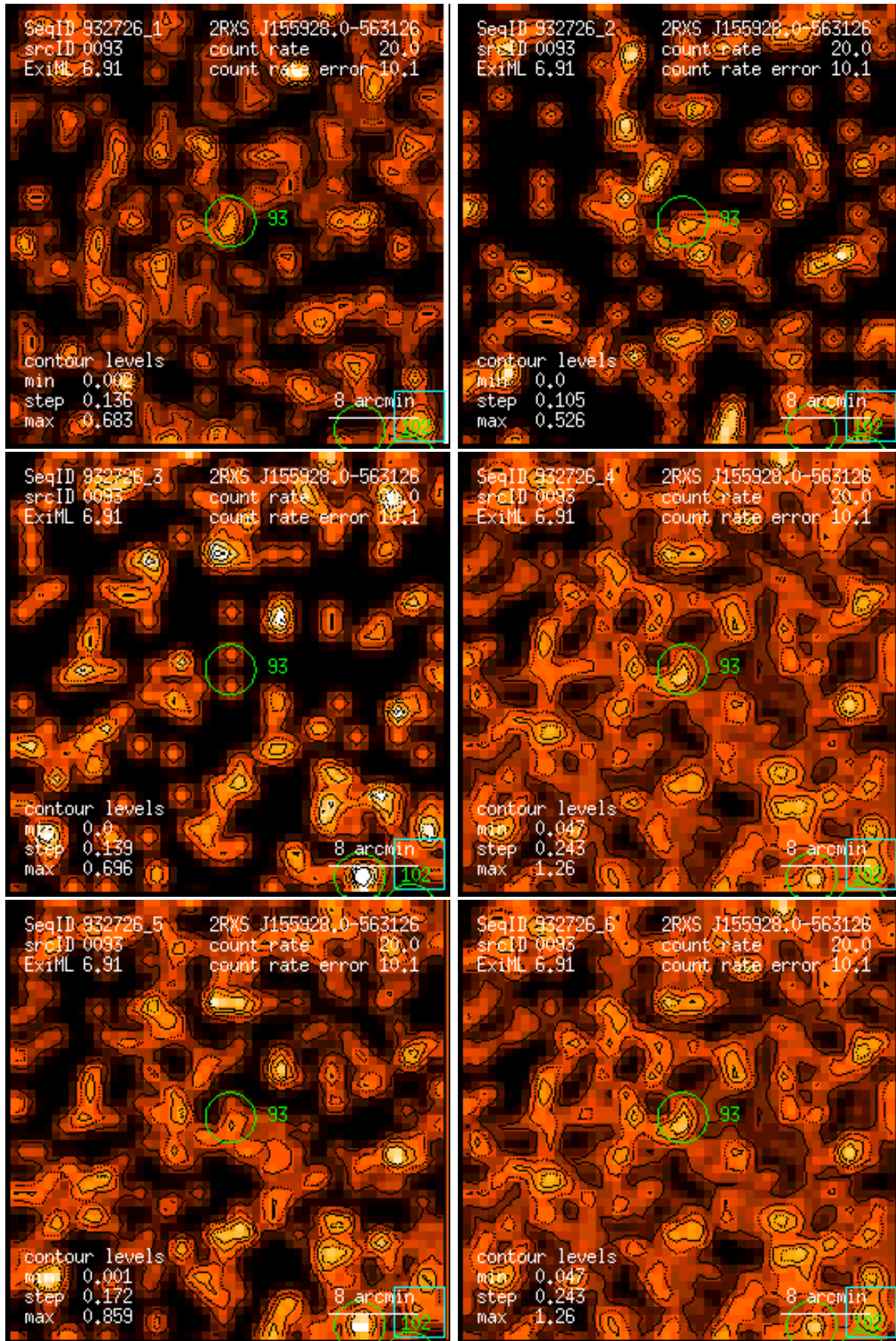
Figure 93: RASS 932726: detection 0093: band rate images, Gaussian filter: (1) PSPC channels 11 – 41, (2) 52 – 90, (3) 91 – 201, (4) 11 – 235, (5) 52 – 201, (6) 11 – 201. Broad band rates in counts/ks. Band rate contour levels in counts/ks/arcmin 2 .
