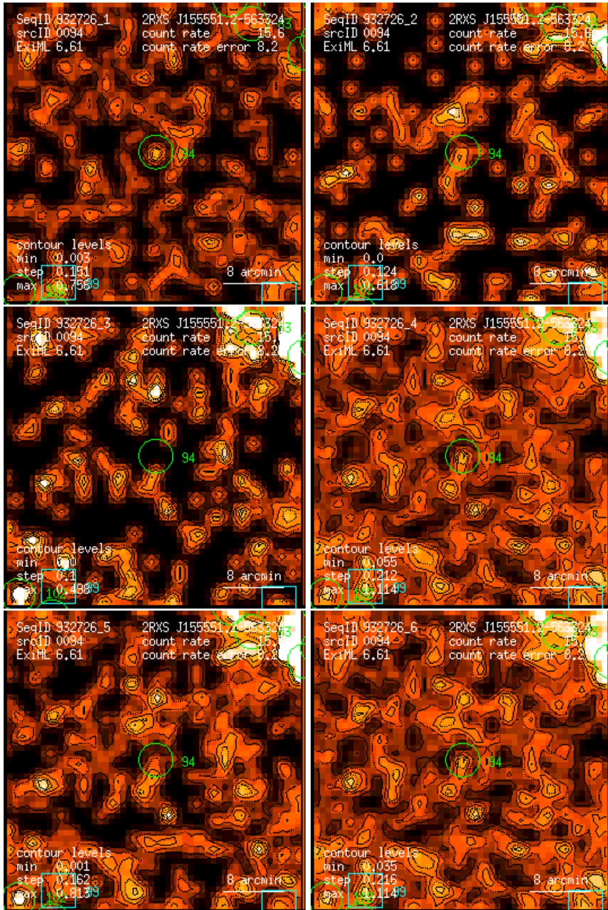
Figure 94: RASS 932726: detection 0094: band rate images, Gaussian filter: (1) PSPC channels 11 – 41, (2) 52 – 90, (3) 91 – 201, (4) 11 – 235, (5) 52 – 201, (6) 11 – 201. Broad band rates in counts/ks. Band rate contour levels in counts/ks/arcmin 2 .
