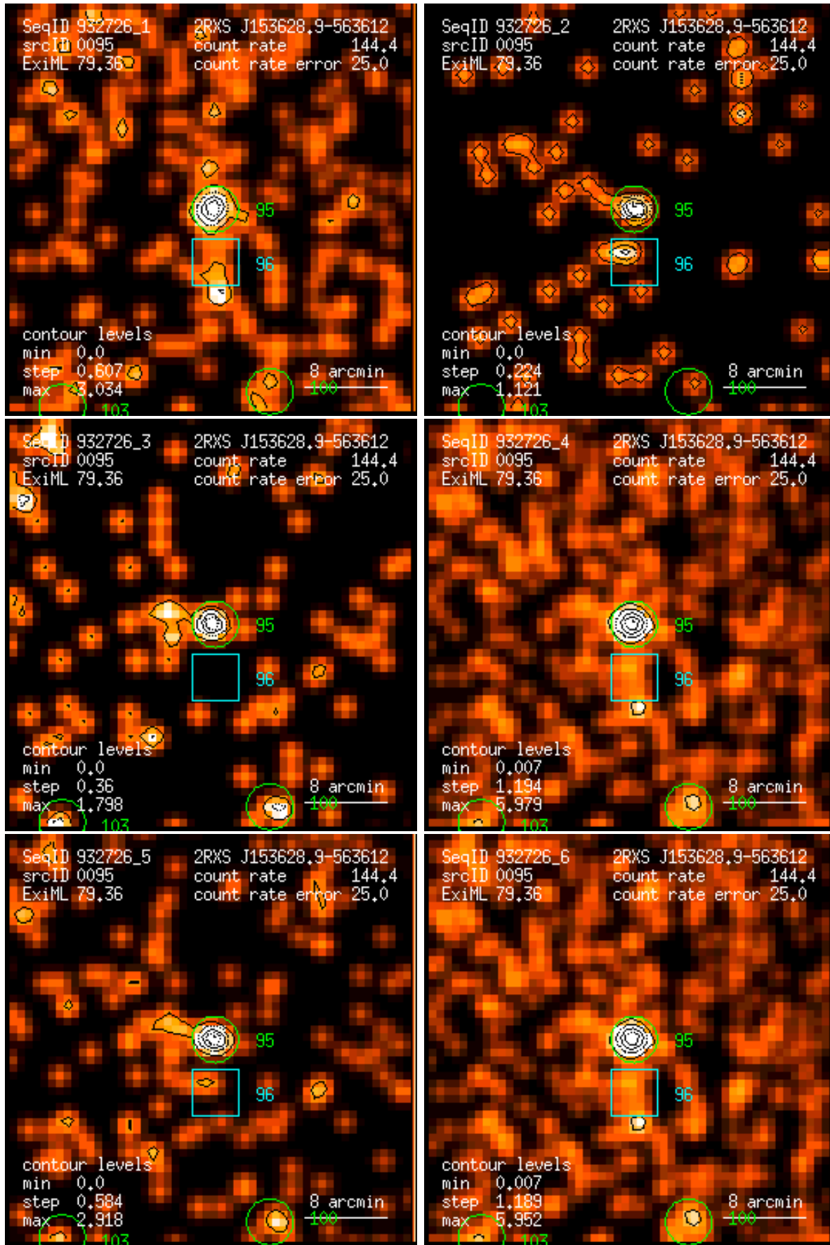
Figure 95: RASS 932726: detection 0095: band rate images, Gaussian filter: (1) PSPC channels 11 – 41, (2) 52 – 90, (3) 91 – 201, (4) 11 – 235, (5) 52 – 201, (6) 11 – 201. Broad band rates in counts/ks. Band rate contour levels in counts/ks/arcmin 2 .
